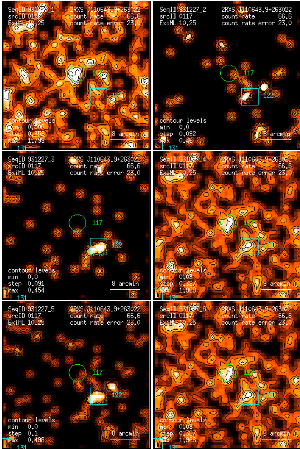
Figure 117: RASS 931227: detection 0117: band rate images, Gaussian filter: (1) PSPC channels 11 – 41, (2) 52 – 90, (3) 91 – 201, (4) 11 – 235, (5) 52 – 201, (6) 11 – 201. Broad band rates in counts/ks. Band rate contour levels in counts/ks/arcmin 2 .
