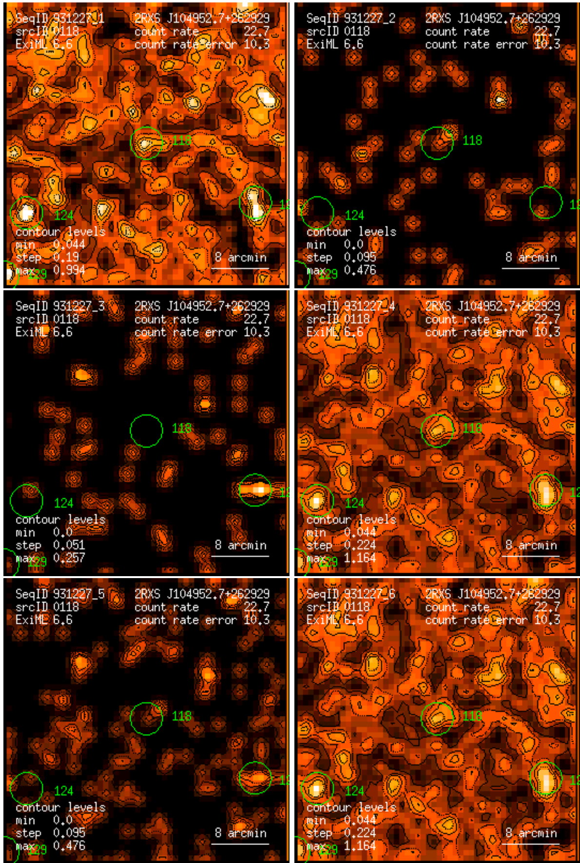
Figure 118: RASS 931227: detection 0118: band rate images, Gaussian filter: (1) PSPC channels 11 – 41, (2) 52 – 90, (3) 91 – 201, (4) 11 – 235, (5) 52 – 201, (6) 11 – 201. Broad band rates in counts/ks. Band rate contour levels in counts/ks/arcmin 2 .
