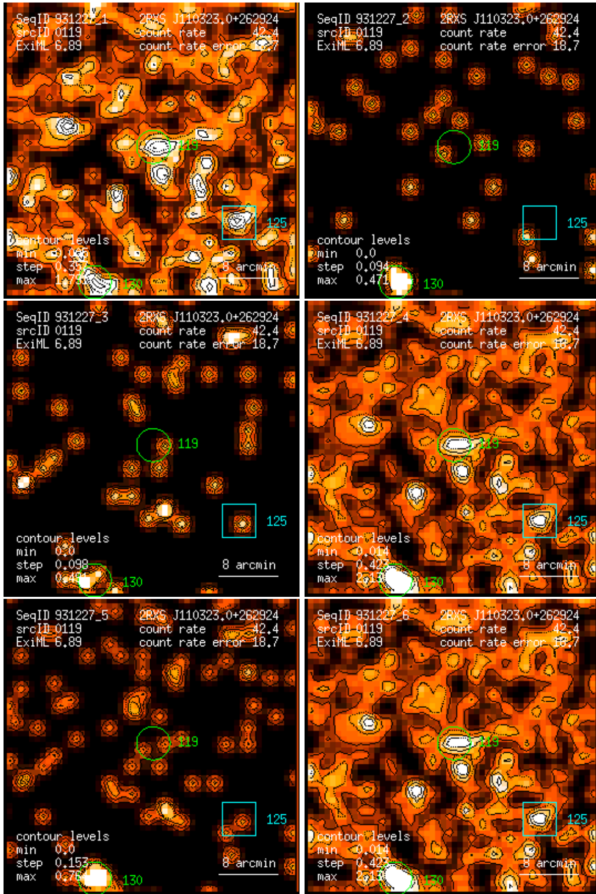
Figure 119: RASS 931227: detection 0119: band rate images, Gaussian filter: (1) PSPC channels 11 – 41, (2) 52 – 90, (3) 91 – 201, (4) 11 – 235, (5) 52 – 201, (6) 11 – 201. Broad band rates in counts/ks. Band rate contour levels in counts/ks/arcmin 2 .
