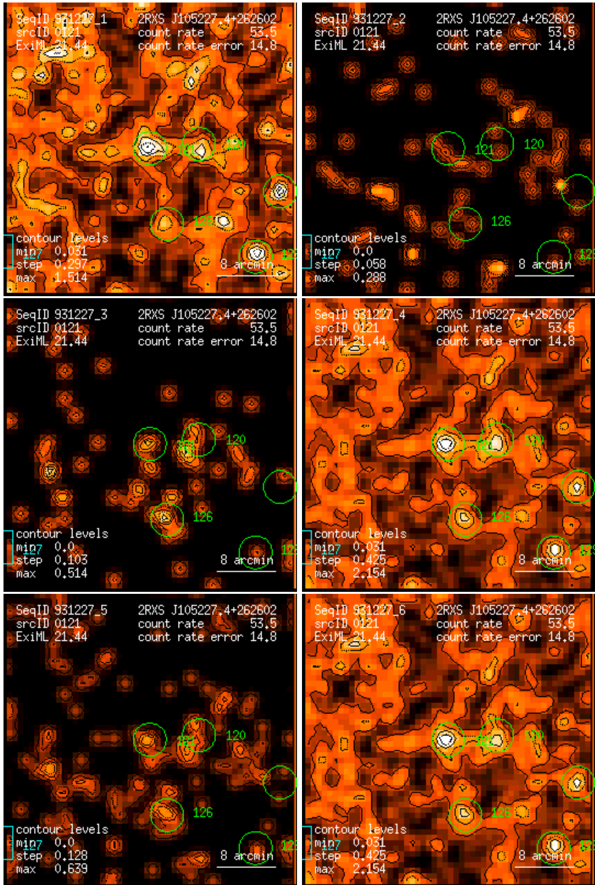
Figure 121: RASS 931227: detection 0121: band rate images, Gaussian filter: (1) PSPC channels 11 – 41, (2) 52 – 90, (3) 91 – 201, (4) 11 – 235, (5) 52 – 201, (6) 11 – 201. Broad band rates in counts/ks. Band rate contour levels in counts/ks/arcmin 2 .
