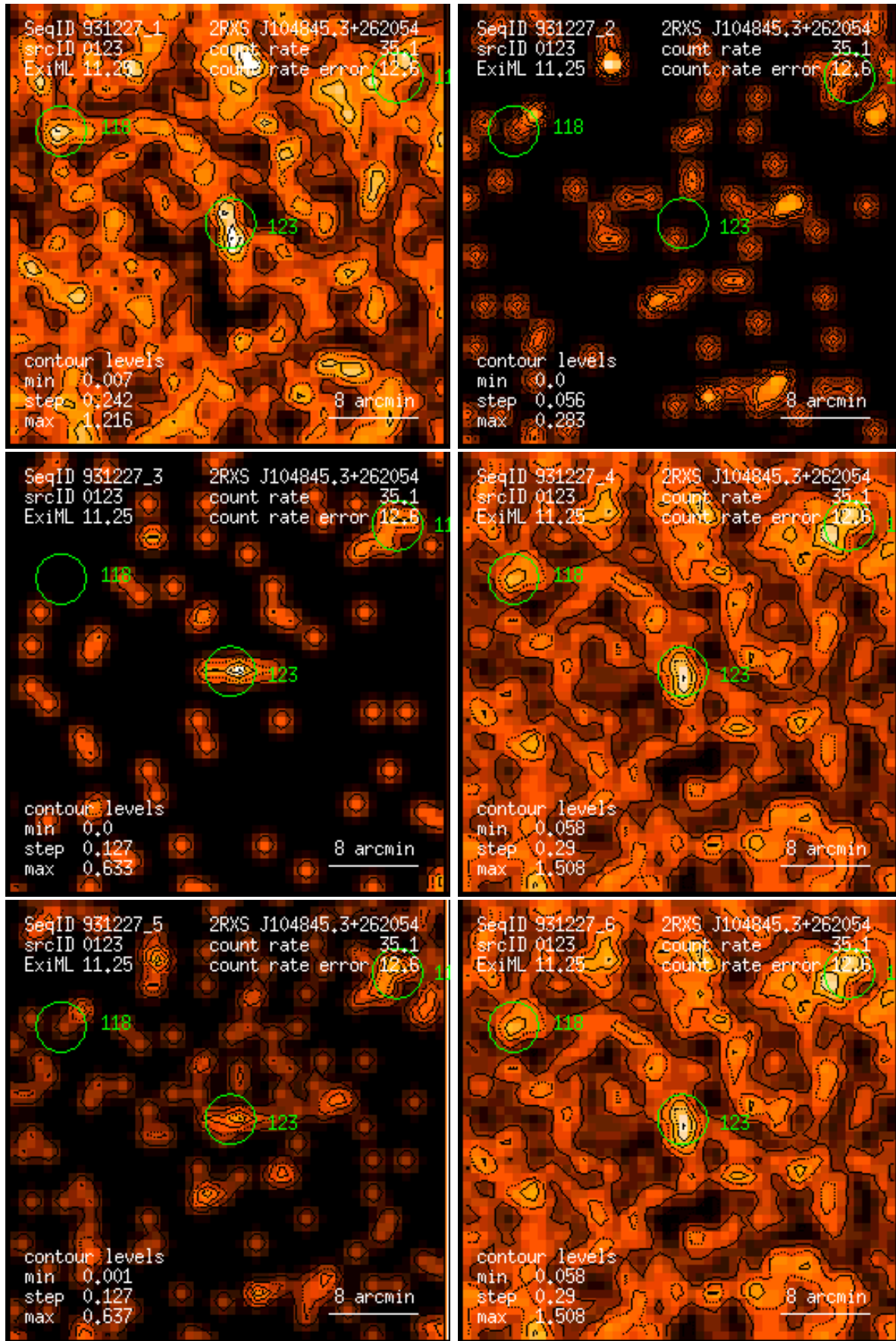
Figure 123: RASS 931227: detection 0123: band rate images, Gaussian filter: (1) PSPC channels 11 – 41, (2) 52 – 90, (3) 91 – 201, (4) 11 – 235, (5) 52 – 201, (6) 11 – 201. Broad band rates in counts/ks. Band rate contour levels in counts/ks/arcmin 2 .
