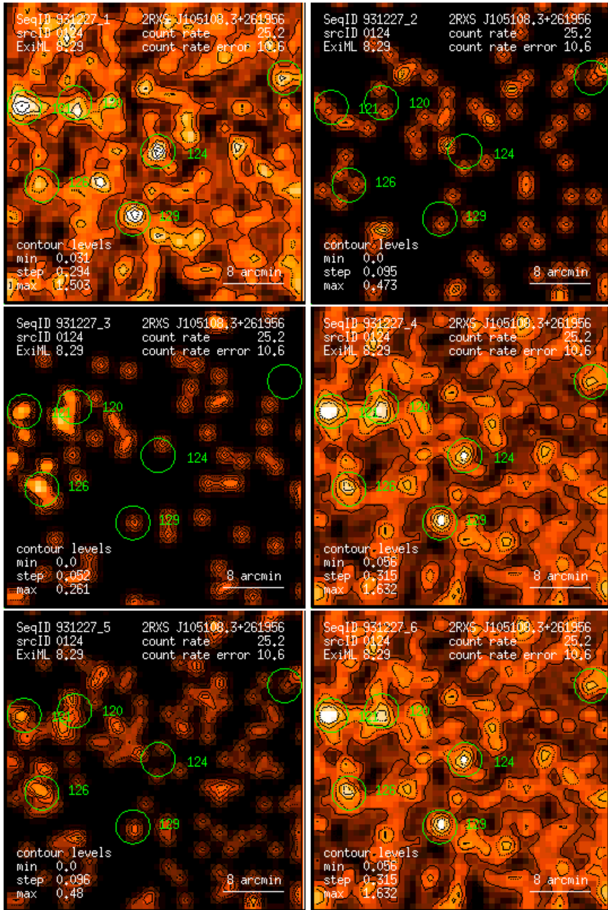
Figure 124: RASS 931227: detection 0124: band rate images, Gaussian filter: (1) PSPC channels 11 – 41, (2) 52 – 90, (3) 91 – 201, (4) 11 – 235, (5) 52 – 201, (6) 11 – 201. Broad band rates in counts/ks. Band rate contour levels in counts/ks/arcmin 2 .
