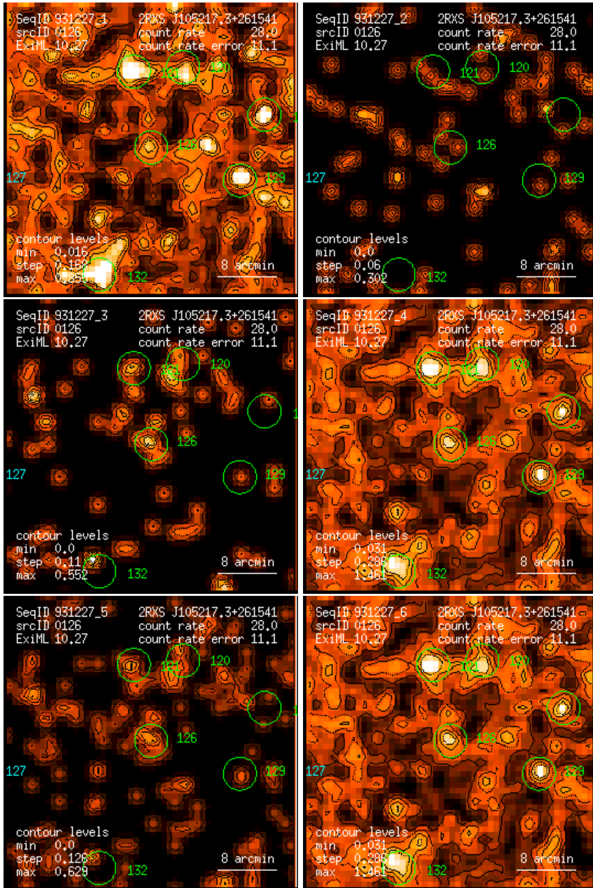
Figure 126: RASS 931227: detection 0126: band rate images, Gaussian filter: (1) PSPC channels 11 – 41, (2) 52 – 90, (3) 91 – 201, (4) 11 – 235, (5) 52 – 201, (6) 11 – 201. Broad band rates in counts/ks. Band rate contour levels in counts/ks/arcmin 2 .
