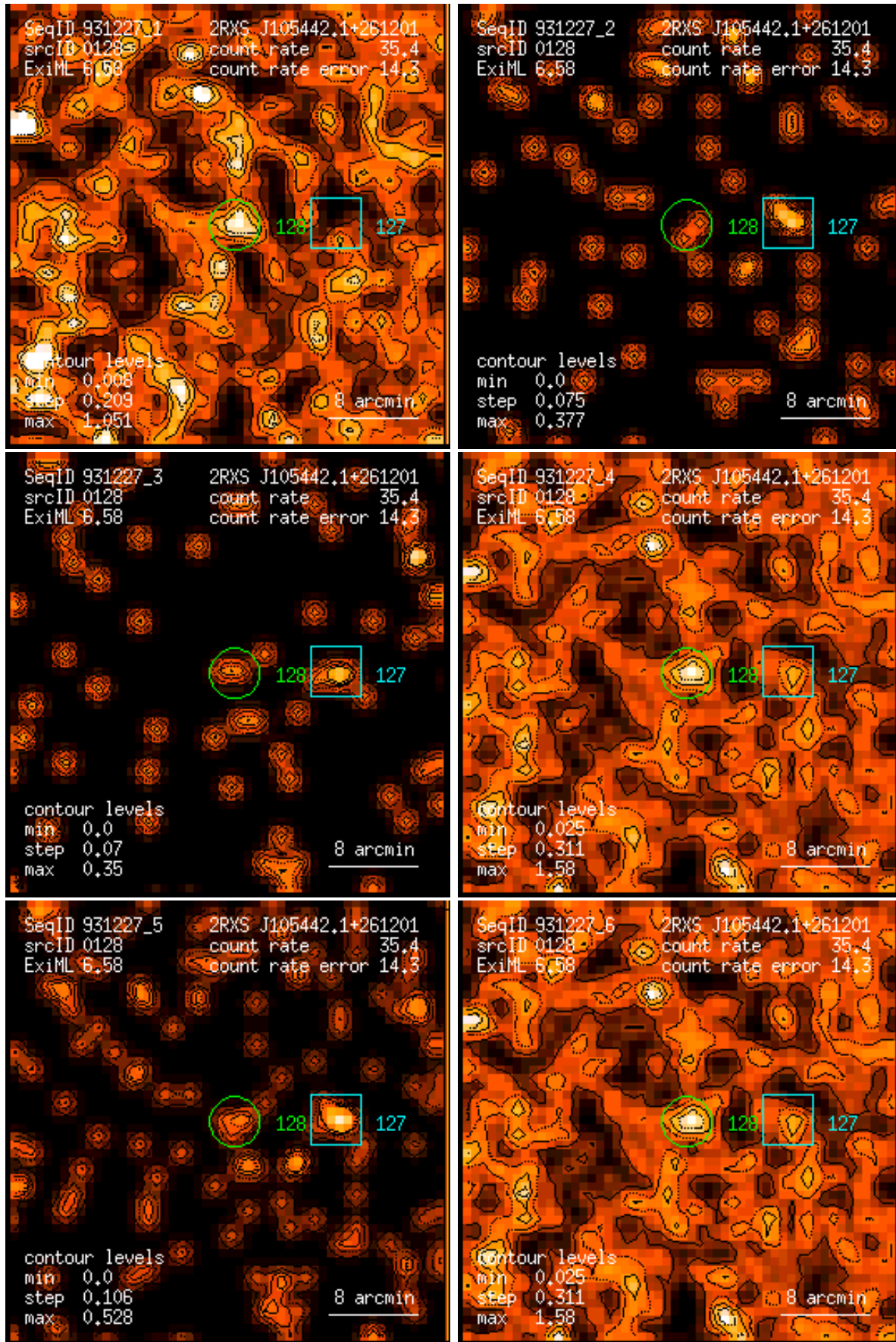
Figure 128: RASS 931227: detection 0128: band rate images, Gaussian filter: (1) PSPC channels 11 – 41, (2) 52 – 90, (3) 91 – 201, (4) 11 – 235, (5) 52 – 201, (6) 11 – 201. Broad band rates in counts/ks. Band rate contour levels in counts/ks/arcmin 2 .
