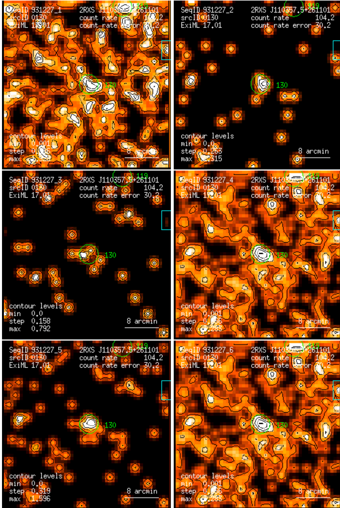
Figure 130: RASS 931227: detection 0130: band rate images, Gaussian filter: (1) PSPC channels 11 – 41, (2) 52 – 90, (3) 91 – 201, (4) 11 – 235, (5) 52 – 201, (6) 11 – 201. Broad band rates in counts/ks. Band rate contour levels in counts/ks/arcmin 2 .
