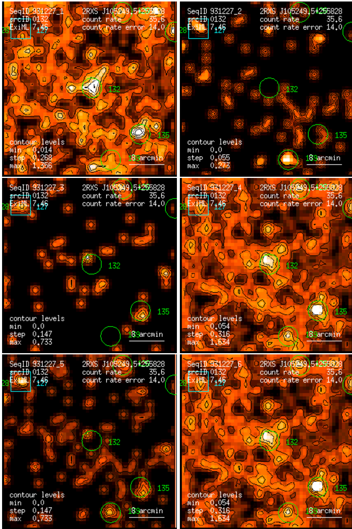
Figure 132: RASS 931227: detection 0132: band rate images, Gaussian filter: (1) PSPC channels 11 – 41, (2) 52 – 90, (3) 91 – 201, (4) 11 – 235, (5) 52 – 201, (6) 11 – 201. Broad band rates in counts/ks. Band rate contour levels in counts/ks/arcmin 2 .
