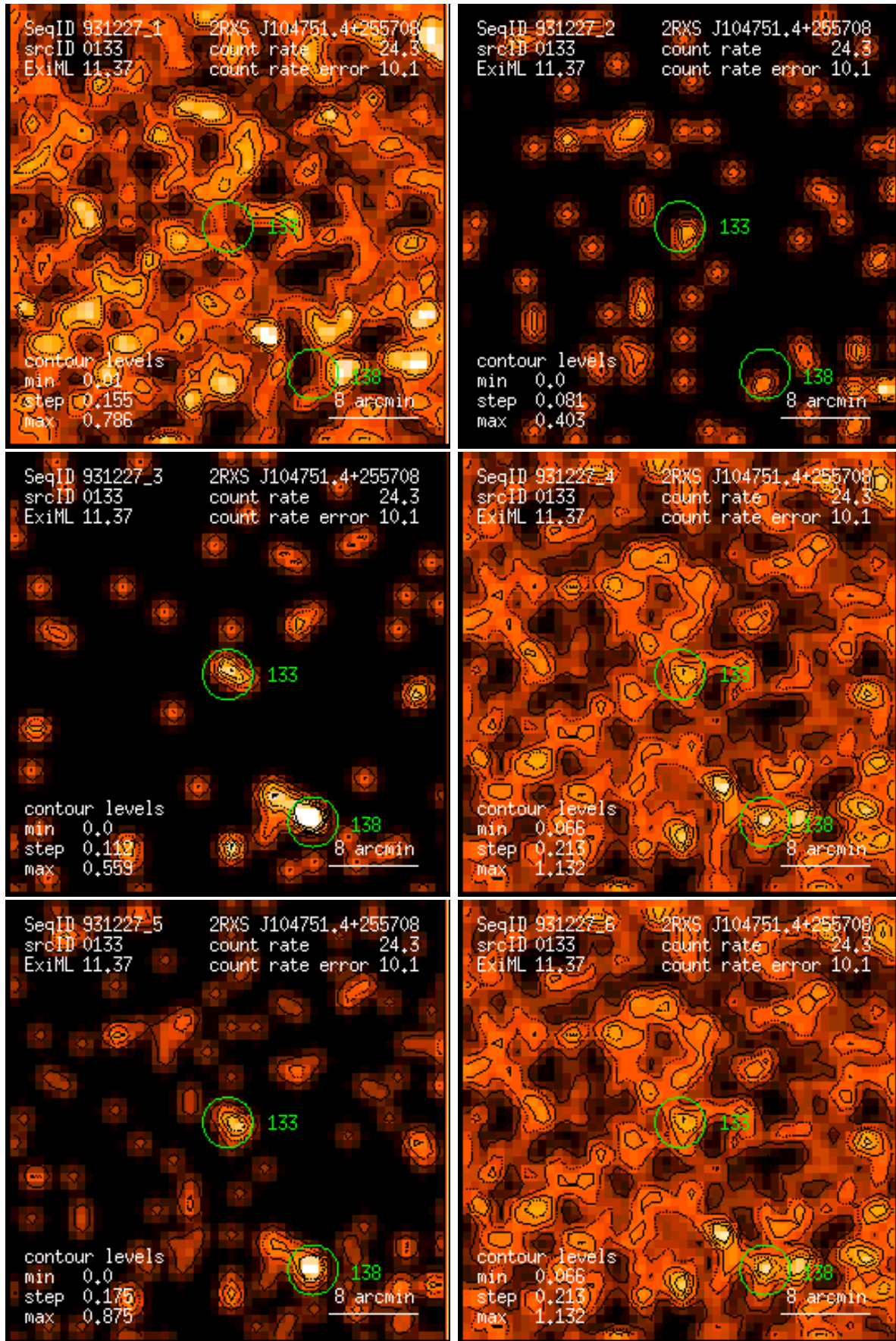
Figure 133: RASS 931227: detection 0133: band rate images, Gaussian filter: (1) PSPC channels 11 – 41, (2) 52 – 90, (3) 91 – 201, (4) 11 – 235, (5) 52 – 201, (6) 11 – 201. Broad band rates in counts/ks. Band rate contour levels in counts/ks/arcmin 2 .
