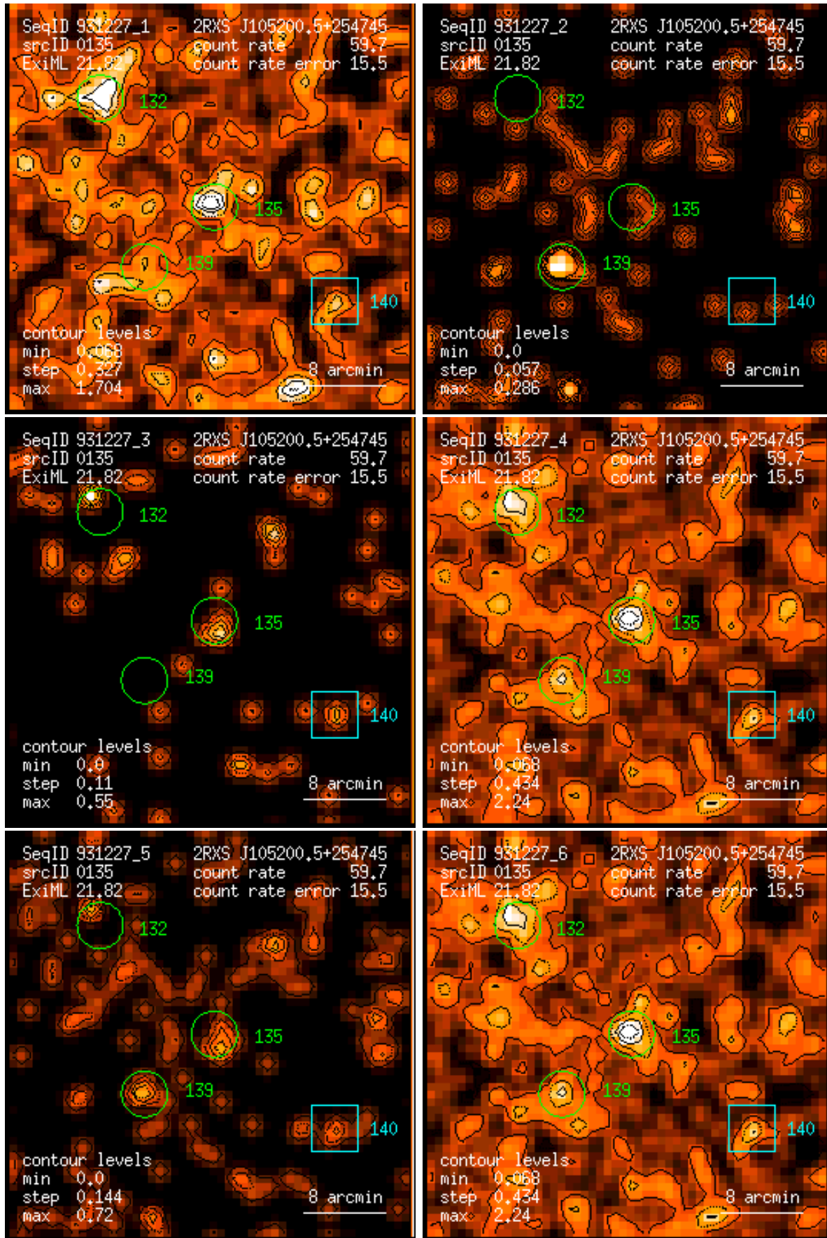
Figure 135: RASS 931227: detection 0135: band rate images, Gaussian filter: (1) PSPC channels 11 – 41, (2) 52 – 90, (3) 91 – 201, (4) 11 – 235, (5) 52 – 201, (6) 11 – 201. Broad band rates in counts/ks. Band rate contour levels in counts/ks/arcmin 2 .
