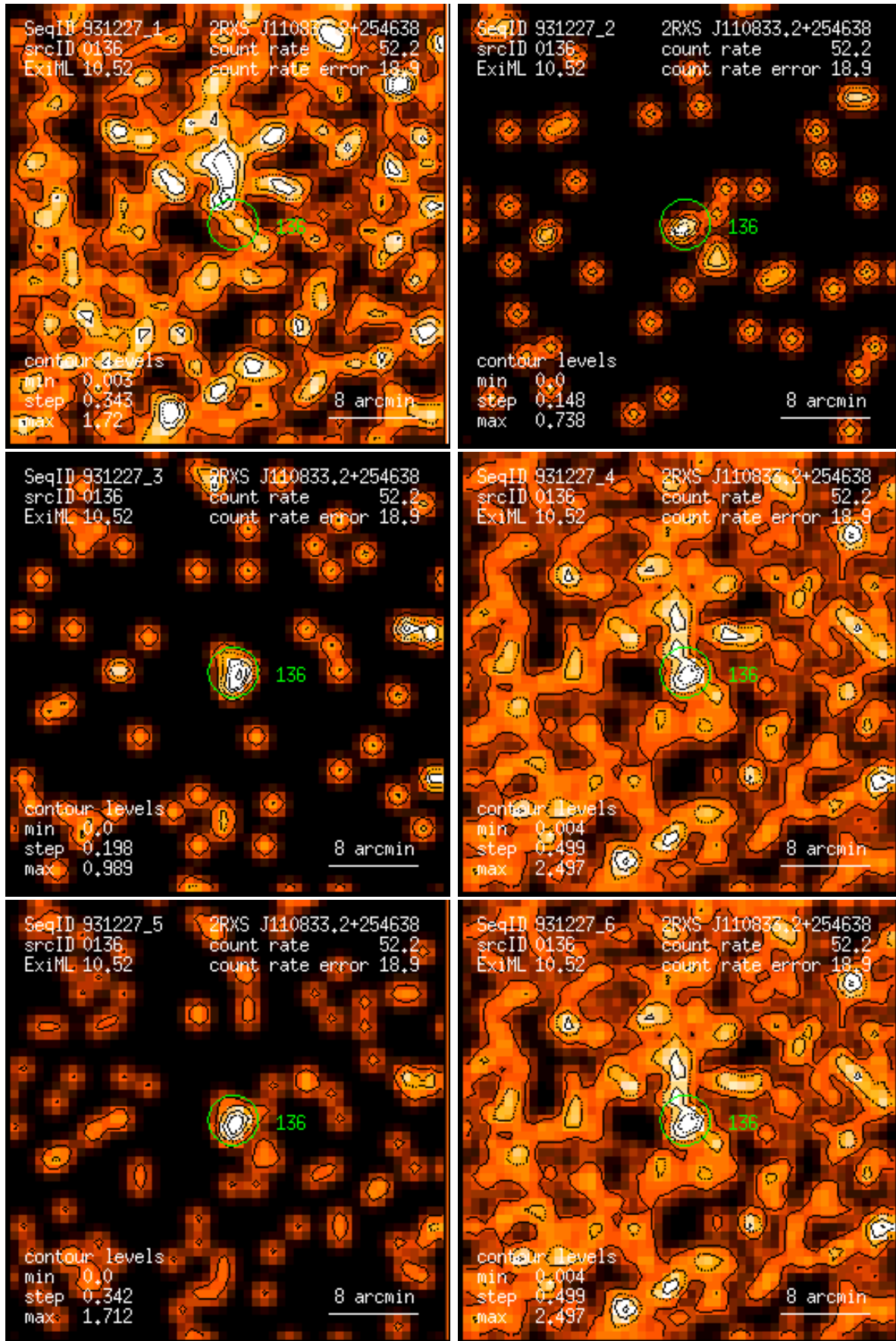
Figure 136: RASS 931227: detection 0136: band rate images, Gaussian filter: (1) PSPC channels 11 – 41, (2) 52 – 90, (3) 91 – 201, (4) 11 – 235, (5) 52 – 201, (6) 11 – 201. Broad band rates in counts/ks. Band rate contour levels in counts/ks/arcmin 2 .
