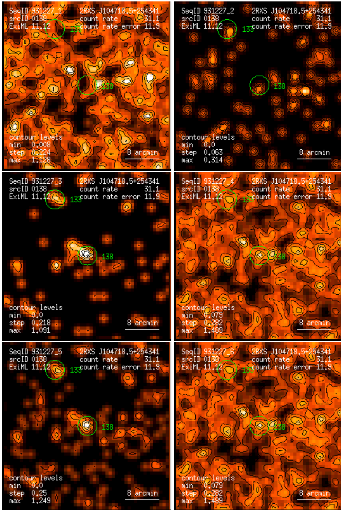
Figure 138: RASS 931227: detection 0138: band rate images, Gaussian filter: (1) PSPC channels 11 – 41, (2) 52 – 90, (3) 91 – 201, (4) 11 – 235, (5) 52 – 201, (6) 11 – 201. Broad band rates in counts/ks. Band rate contour levels in counts/ks/arcmin 2 .
