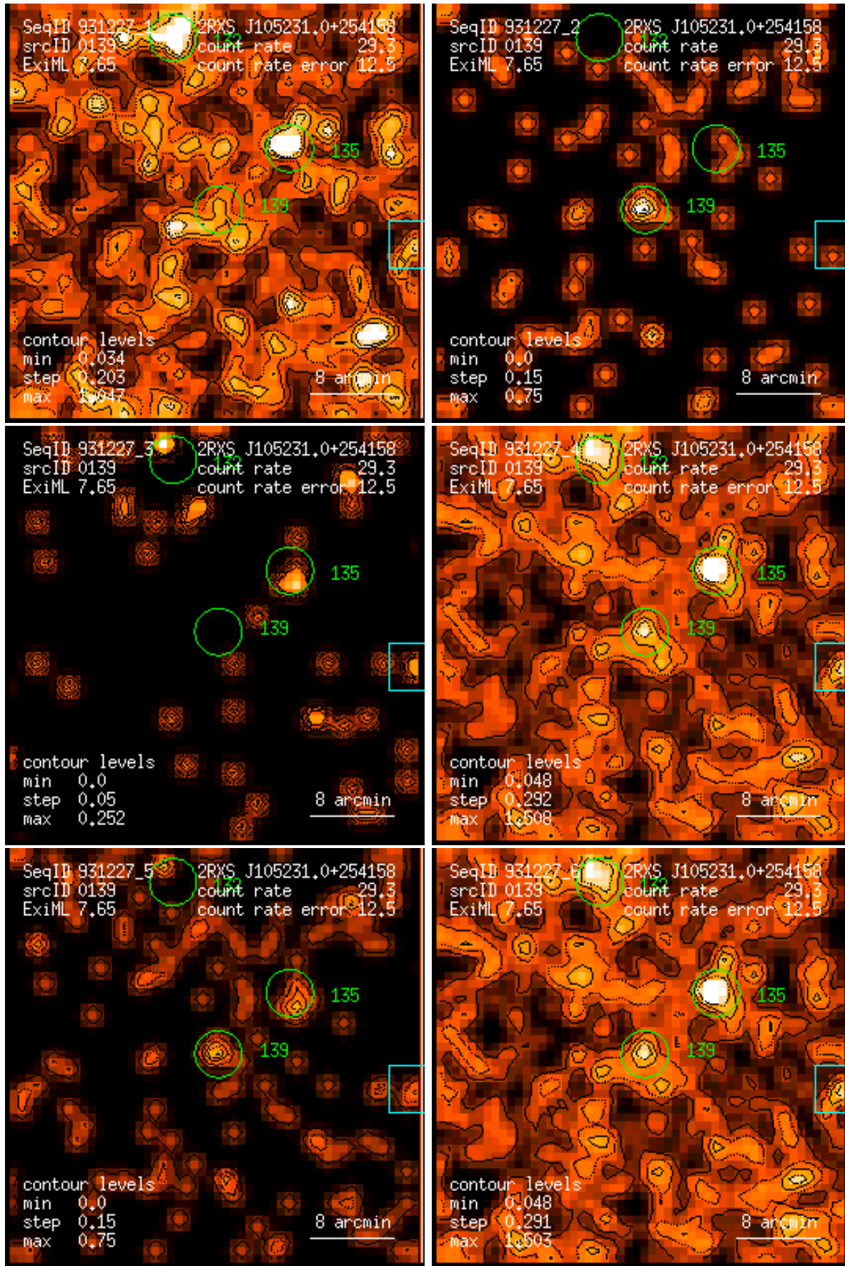
Figure 139: RASS 931227: detection 0139: band rate images, Gaussian filter: (1) PSPC channels 11 – 41, (2) 52 – 90, (3) 91 – 201, (4) 11 – 235, (5) 52 – 201, (6) 11 – 201. Broad band rates in counts/ks. Band rate contour levels in counts/ks/arcmin 2 .
