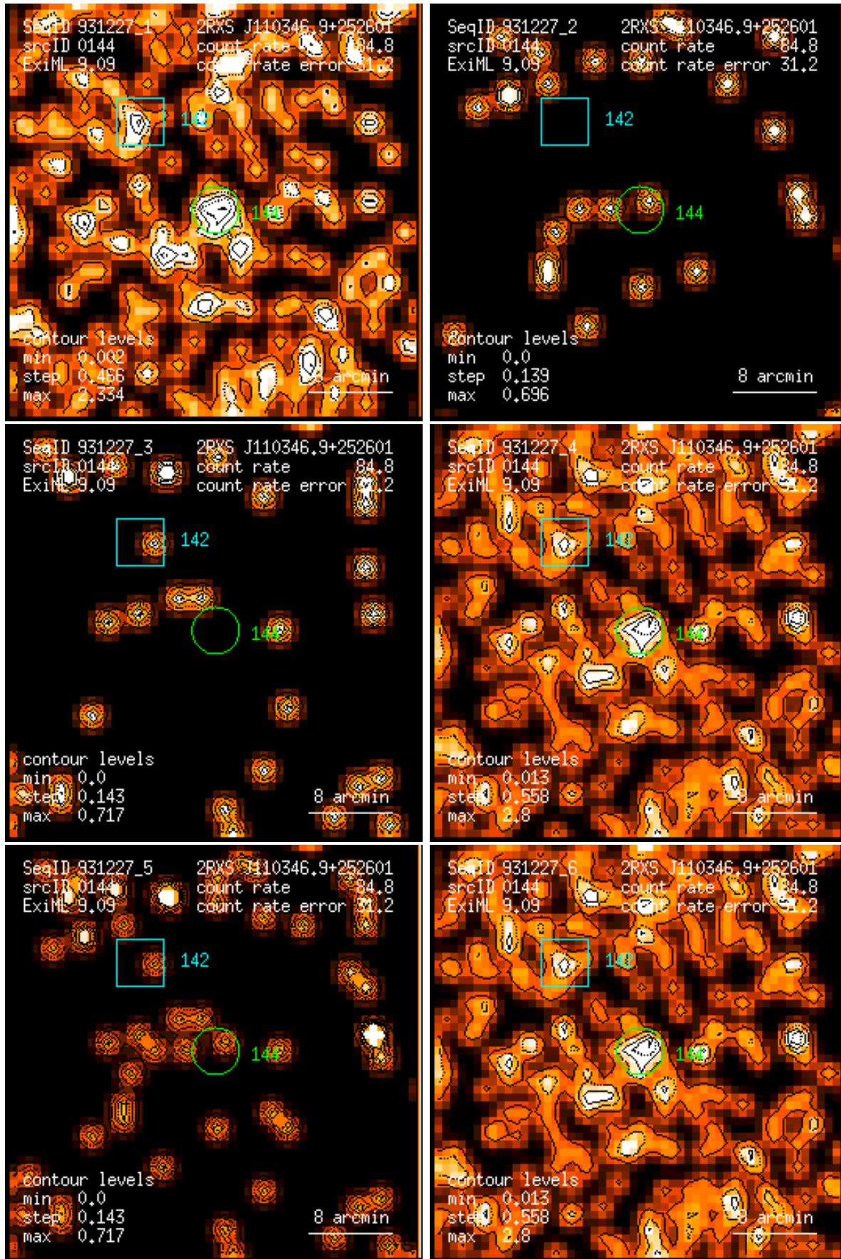
Figure 144: RASS 931227: detection 0144: band rate images, Gaussian filter: (1) PSPC channels 11 – 41, (2) 52 – 90, (3) 91 – 201, (4) 11 – 235, (5) 52 – 201, (6) 11 – 201. Broad band rates in counts/ks. Band rate contour levels in counts/ks/arcmin 2 .
