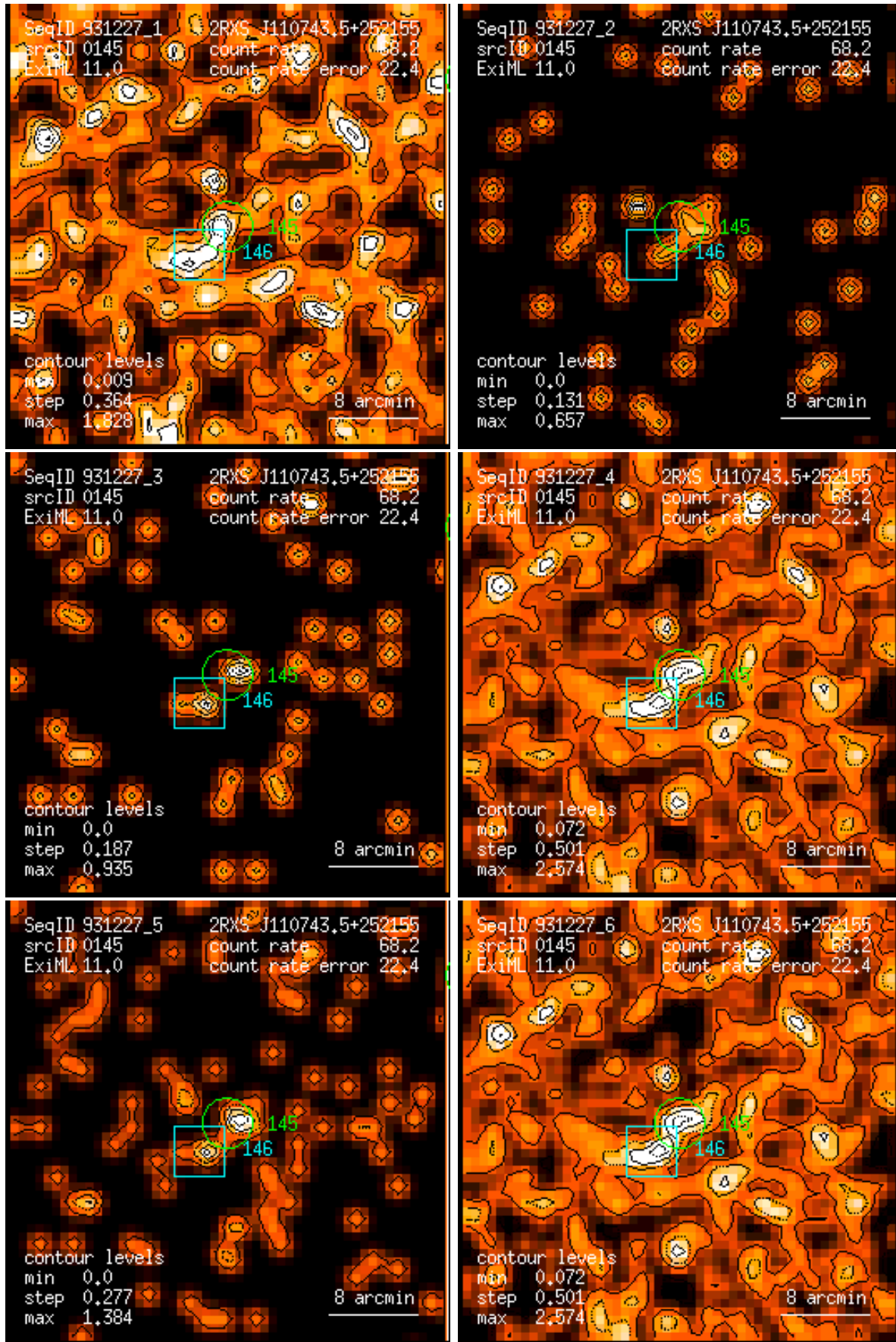
Figure 145: RASS 931227: detection 0145: band rate images, Gaussian filter: (1) PSPC channels 11 – 41, (2) 52 – 90, (3) 91 – 201, (4) 11 – 235, (5) 52 – 201, (6) 11 – 201. Broad band rates in counts/ks. Band rate contour levels in counts/ks/arcmin 2 .
