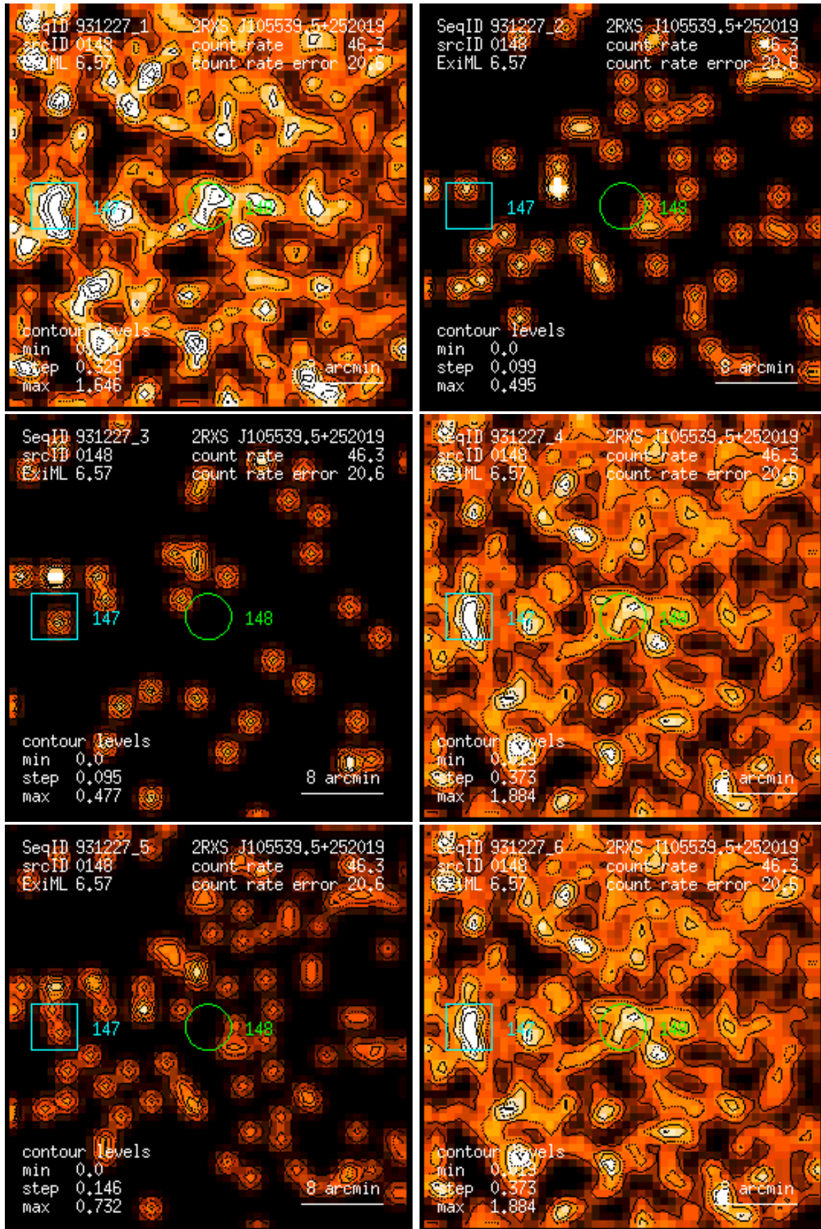
Figure 148: RASS 931227: detection 0148: band rate images, Gaussian filter: (1) PSPC channels 11 – 41, (2) 52 – 90, (3) 91 – 201, (4) 11 – 235, (5) 52 – 201, (6) 11 – 201. Broad band rates in counts/ks. Band rate contour levels in counts/ks/arcmin 2 .
