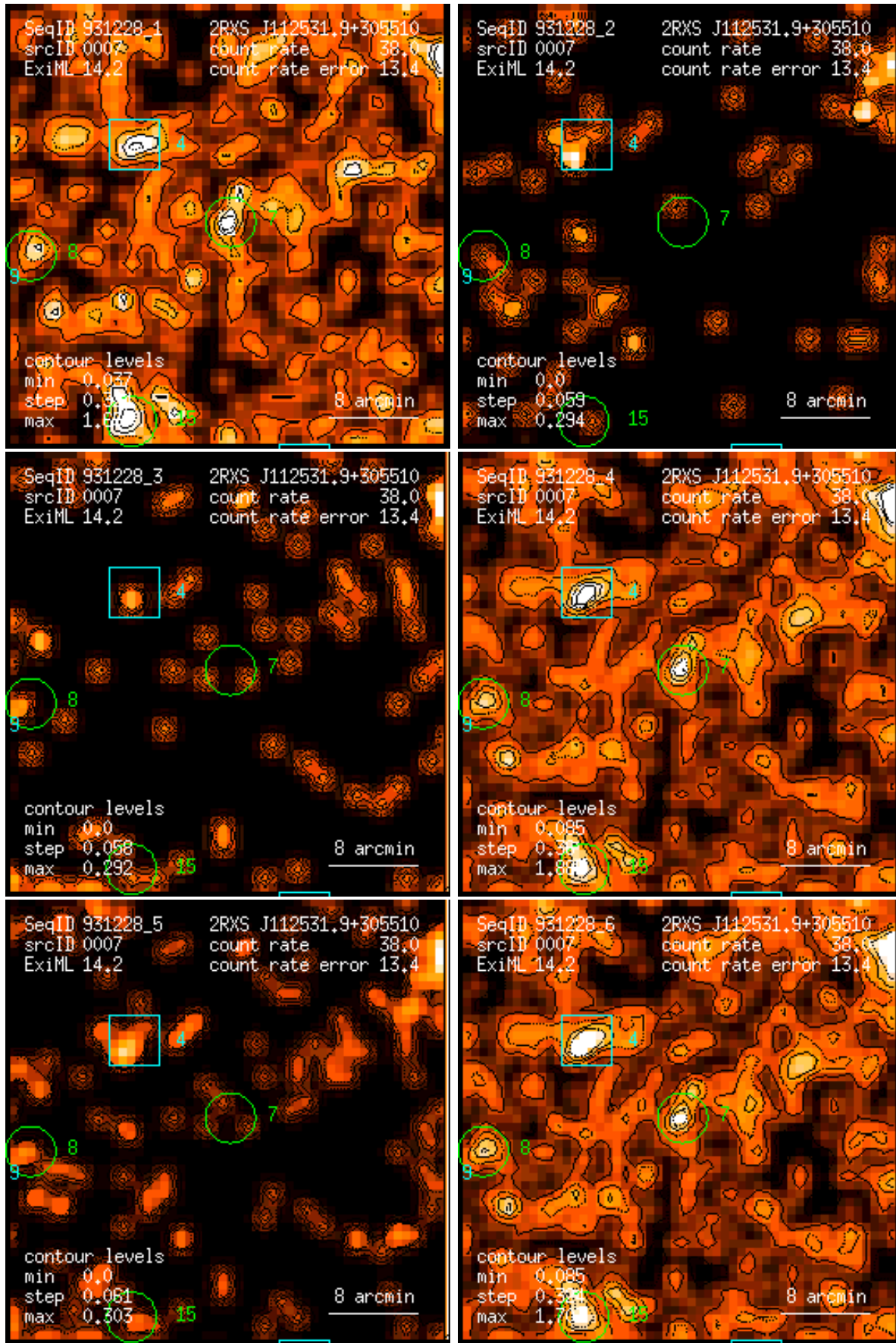
Figure 7: RASS 931228: detection 0007: band rate images, Gaussian filter: (1) PSPC channels 11 – 41, (2) 52 – 90, (3) 91 – 201, (4) 11 – 235, (5) 52 – 201, (6) 11 – 201. Broad band rates in counts/ks. Band rate contour levels in counts/ks/arcmin 2 .
