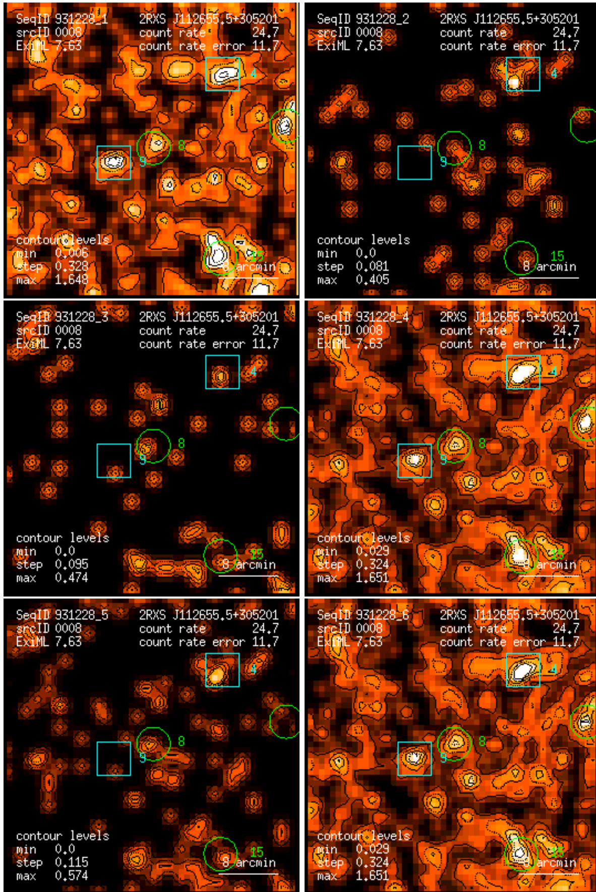
Figure 8: RASS 931228: detection 0008: band rate images, Gaussian filter: (1) PSPC channels 11 – 41, (2) 52 – 90, (3) 91 – 201, (4) 11 – 235, (5) 52 – 201, (6) 11 – 201. Broad band rates in counts/ks. Band rate contour levels in counts/ks/arcmin 2 .
