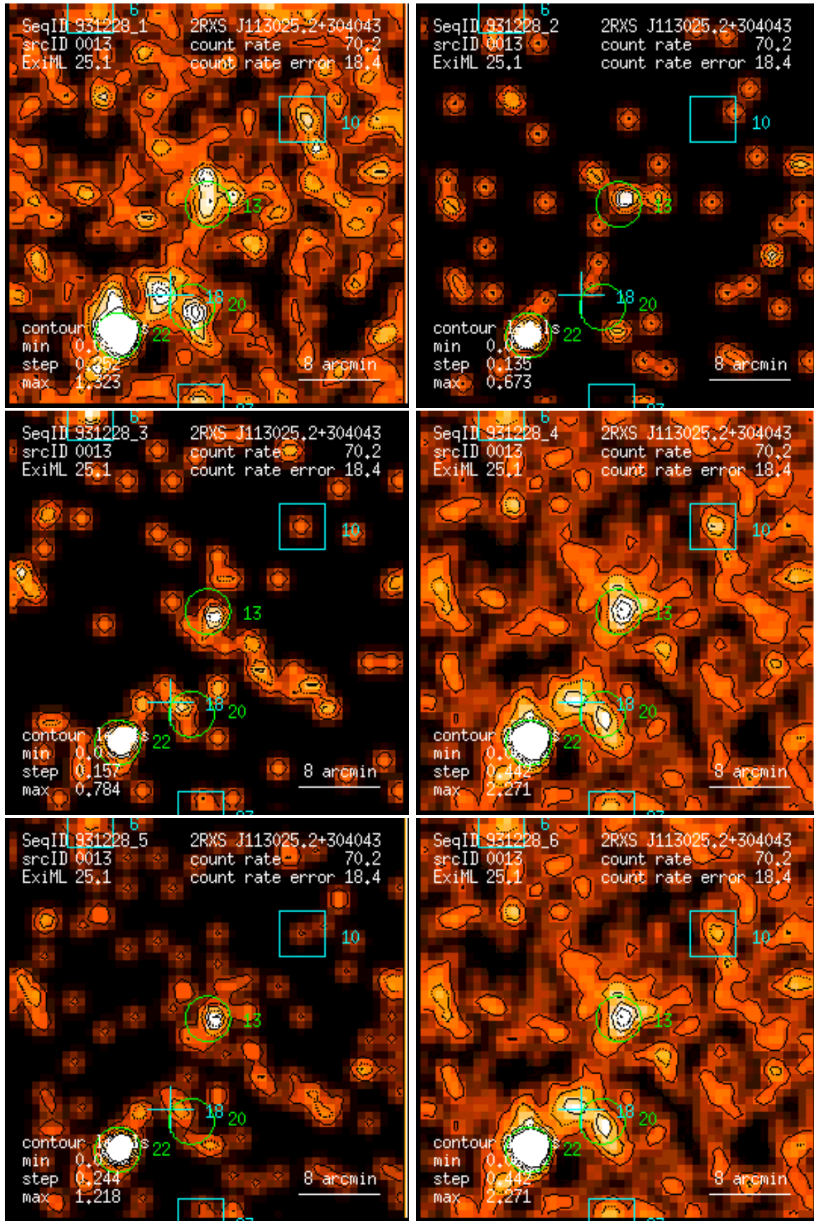
Figure 13: RASS 931228: detection 0013: band rate images, Gaussian filter: (1) PSPC channels 11 – 41, (2) 52 – 90, (3) 91 – 201, (4) 11 – 235, (5) 52 – 201, (6) 11 – 201. Broad band rates in counts/ks. Band rate contour levels in counts/ks/arcmin 2 .
