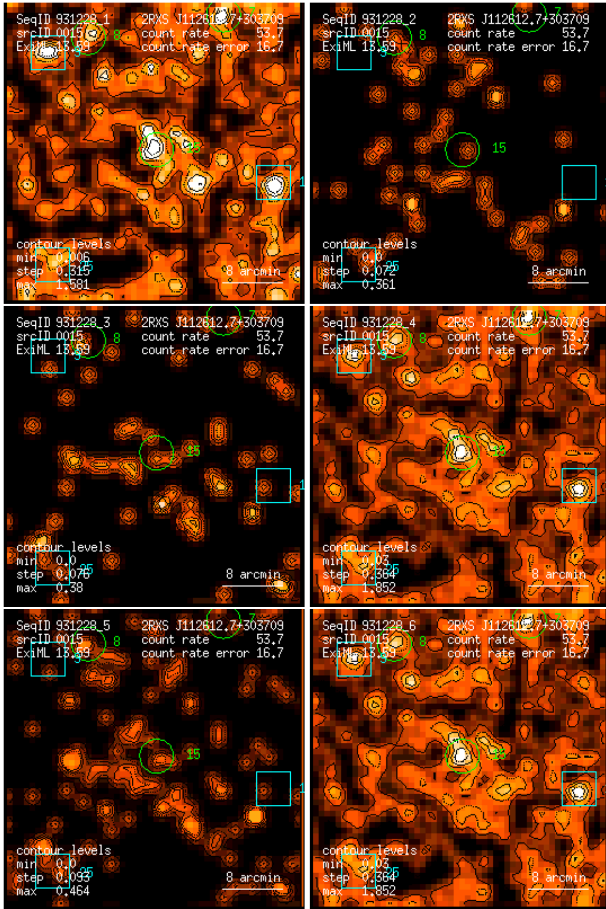
Figure 15: RASS 931228: detection 0015: band rate images, Gaussian filter: (1) PSPC channels 11 – 41, (2) 52 – 90, (3) 91 – 201, (4) 11 – 235, (5) 52 – 201, (6) 11 – 201. Broad band rates in counts/ks. Band rate contour levels in counts/ks/arcmin 2 .
