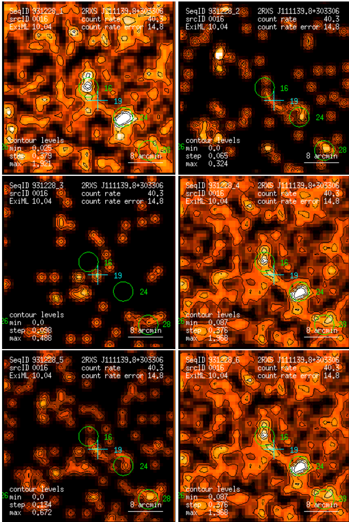
Figure 16: RASS 931228: detection 0016: band rate images, Gaussian filter: (1) PSPC channels 11 – 41, (2) 52 – 90, (3) 91 – 201, (4) 11 – 235, (5) 52 – 201, (6) 11 – 201. Broad band rates in counts/ks. Band rate contour levels in counts/ks/arcmin 2 .
