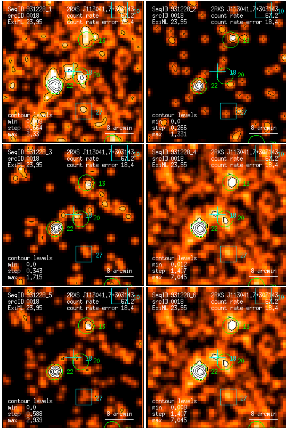
Figure 18: RASS 931228: detection 0018: band rate images, Gaussian filter: (1) PSPC channels 11 – 41, (2) 52 – 90, (3) 91 – 201, (4) 11 – 235, (5) 52 – 201, (6) 11 – 201. Broad band rates in counts/ks. Band rate contour levels in counts/ks/arcmin 2 .
