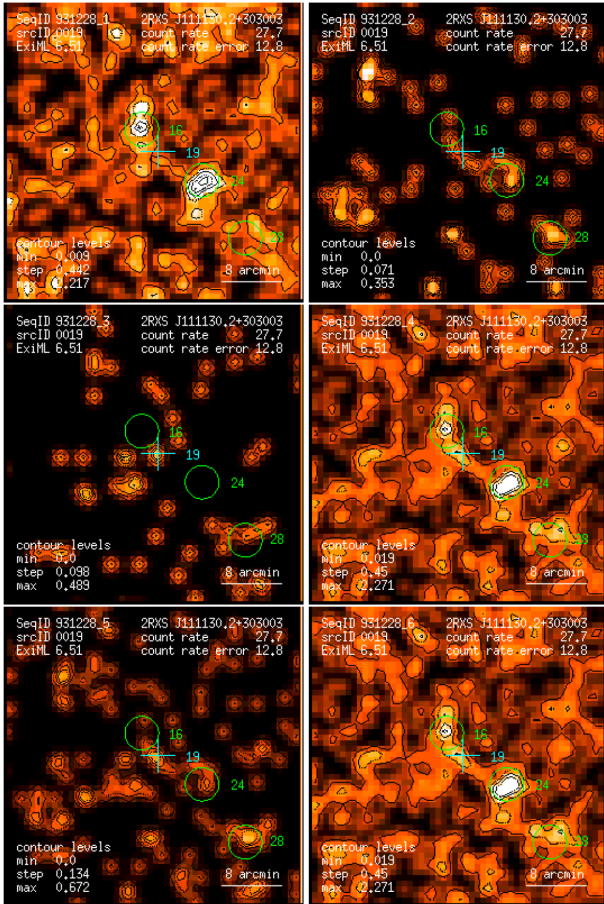
Figure 19: RASS 931228: detection 0019: band rate images, Gaussian filter: (1) PSPC channels 11 – 41, (2) 52 – 90, (3) 91 – 201, (4) 11 – 235, (5) 52 – 201, (6) 11 – 201. Broad band rates in counts/ks. Band rate contour levels in counts/ks/arcmin 2 .
