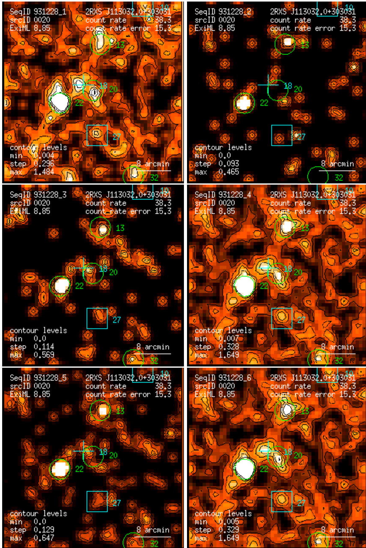
Figure 20: RASS 931228: detection 0020: band rate images, Gaussian filter: (1) PSPC channels 11 – 41, (2) 52 – 90, (3) 91 – 201, (4) 11 – 235, (5) 52 – 201, (6) 11 – 201. Broad band rates in counts/ks. Band rate contour levels in counts/ks/arcmin 2 .
