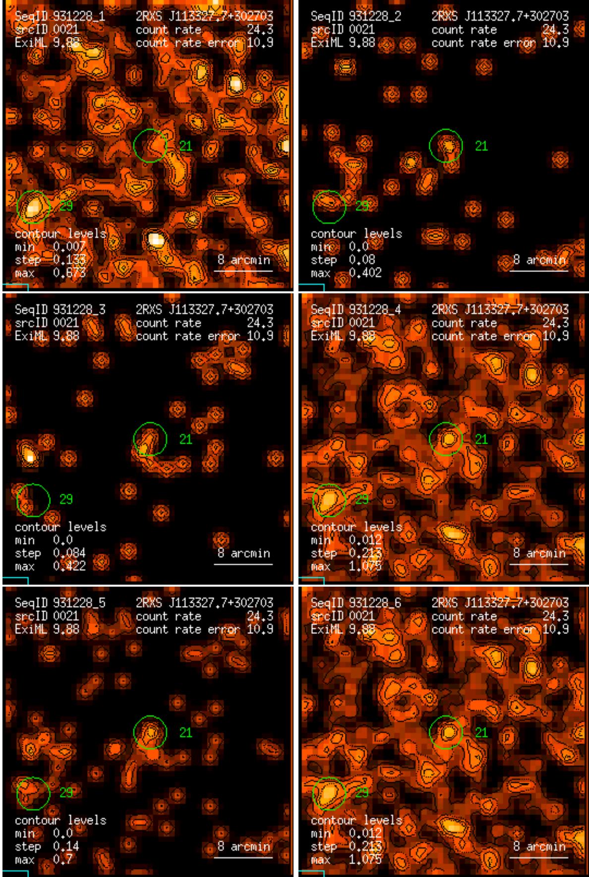
Figure 21: RASS 931228: detection 0021: band rate images, Gaussian filter: (1) PSPC channels 11 – 41, (2) 52 – 90, (3) 91 – 201, (4) 11 – 235, (5) 52 – 201, (6) 11 – 201. Broad band rates in counts/ks. Band rate contour levels in counts/ks/arcmin 2 .
