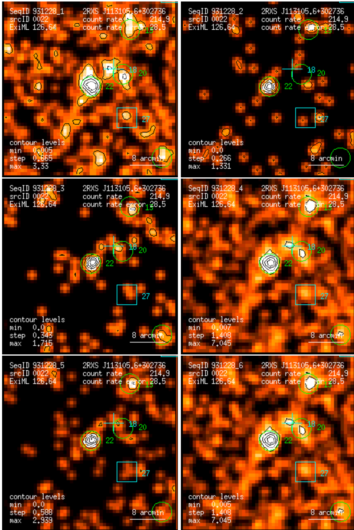
Figure 22: RASS 931228: detection 0022: band rate images, Gaussian filter: (1) PSPC channels 11 – 41, (2) 52 – 90, (3) 91 – 201, (4) 11 – 235, (5) 52 – 201, (6) 11 – 201. Broad band rates in counts/ks. Band rate contour levels in counts/ks/arcmin 2 .
