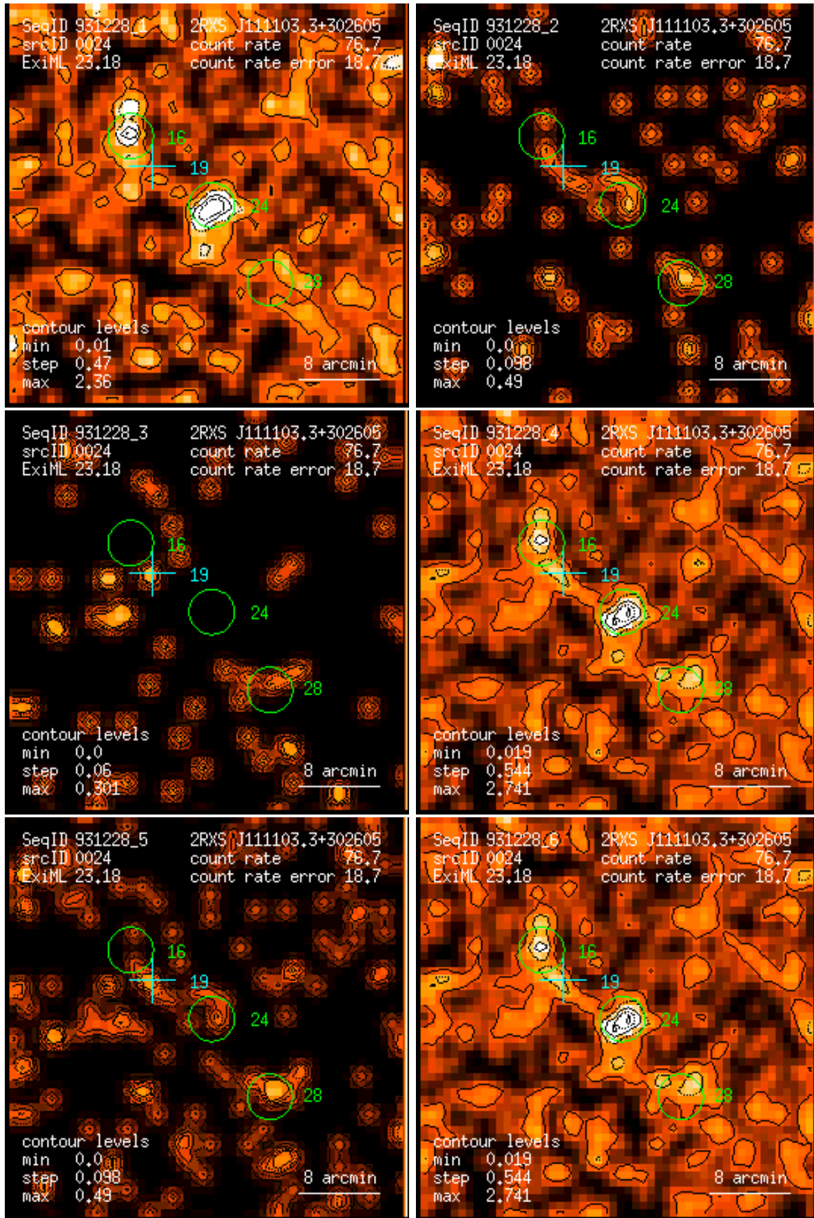
Figure 24: RASS 931228: detection 0024: band rate images, Gaussian filter: (1) PSPC channels 11 – 41, (2) 52 – 90, (3) 91 – 201, (4) 11 – 235, (5) 52 – 201, (6) 11 – 201. Broad band rates in counts/ks. Band rate contour levels in counts/ks/arcmin 2 .
