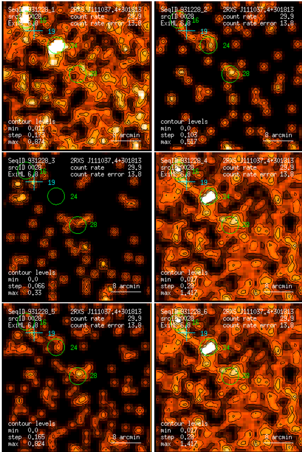
Figure 28: RASS 931228: detection 0028: band rate images, Gaussian filter: (1) PSPC channels 11 – 41, (2) 52 – 90, (3) 91 – 201, (4) 11 – 235, (5) 52 – 201, (6) 11 – 201. Broad band rates in counts/ks. Band rate contour levels in counts/ks/arcmin 2 .
