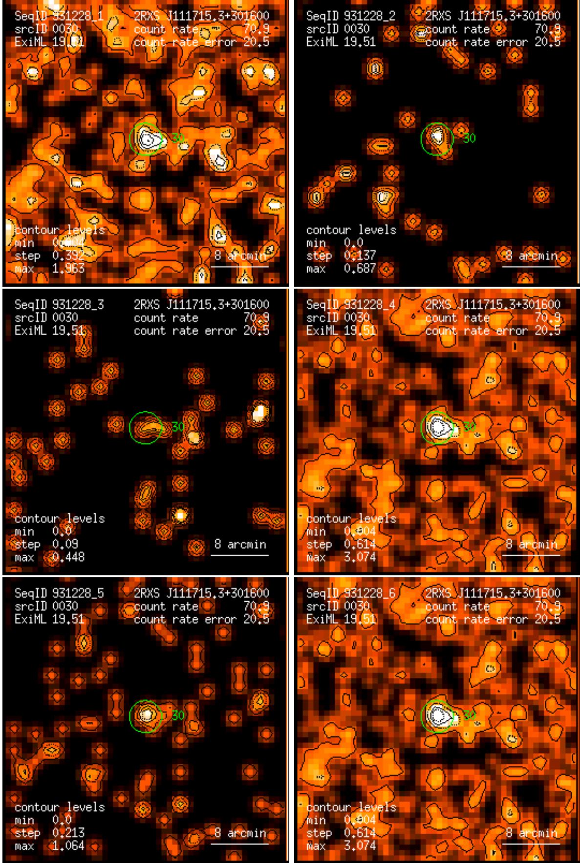
Figure 30: RASS 931228: detection 0030: band rate images, Gaussian filter: (1) PSPC channels 11 – 41, (2) 52 – 90, (3) 91 – 201, (4) 11 – 235, (5) 52 – 201, (6) 11 – 201. Broad band rates in counts/ks. Band rate contour levels in counts/ks/arcmin 2 .
