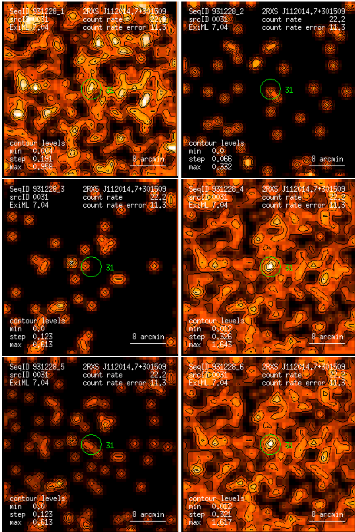
Figure 31: RASS 931228: detection 0031: band rate images, Gaussian filter: (1) PSPC channels 11 – 41, (2) 52 – 90, (3) 91 – 201, (4) 11 – 235, (5) 52 – 201, (6) 11 – 201. Broad band rates in counts/ks. Band rate contour levels in counts/ks/arcmin 2 .
