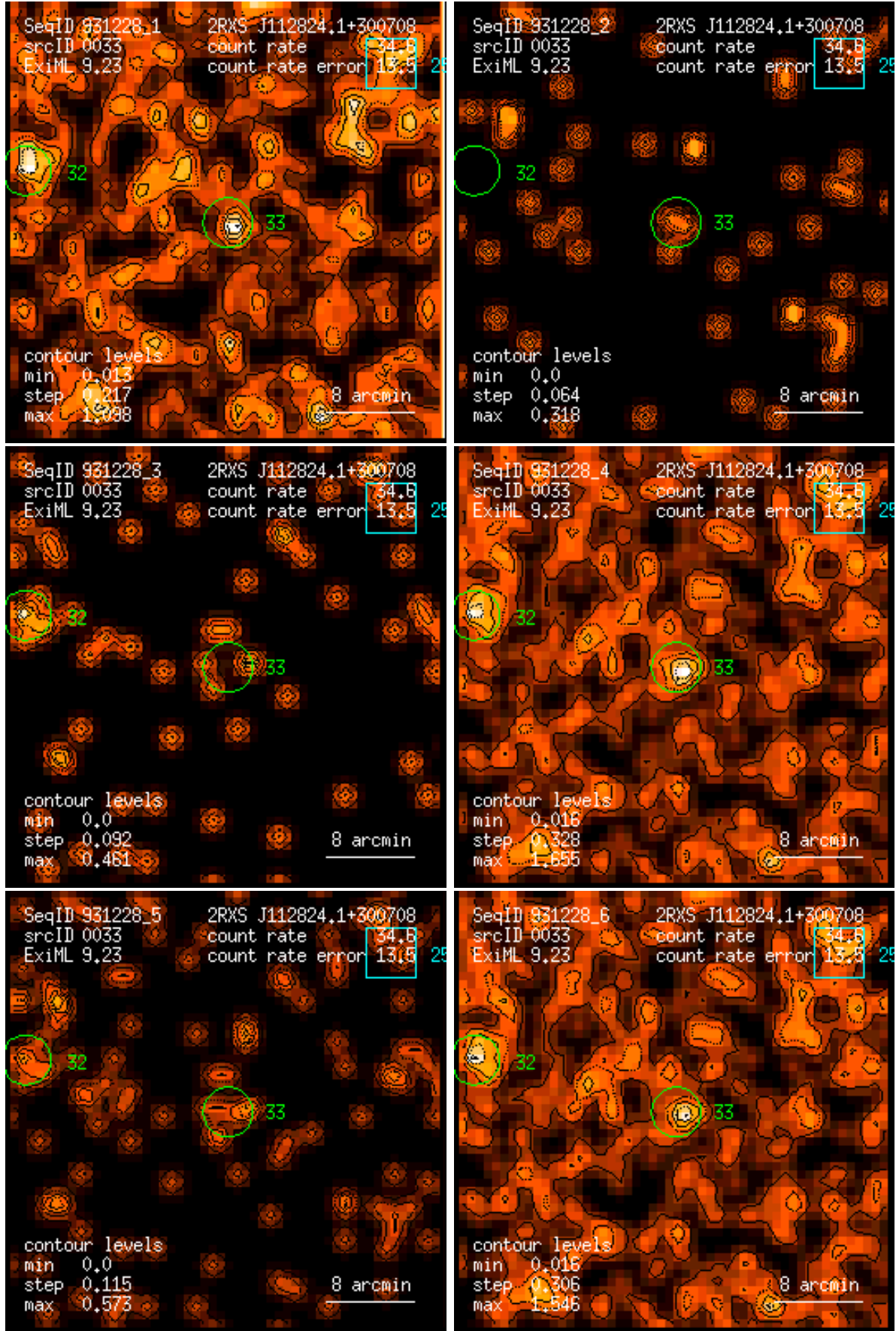
Figure 33: RASS 931228: detection 0033: band rate images, Gaussian filter: (1) PSPC channels 11 – 41, (2) 52 – 90, (3) 91 – 201, (4) 11 – 235, (5) 52 – 201, (6) 11 – 201. Broad band rates in counts/ks. Band rate contour levels in counts/ks/arcmin 2 .
