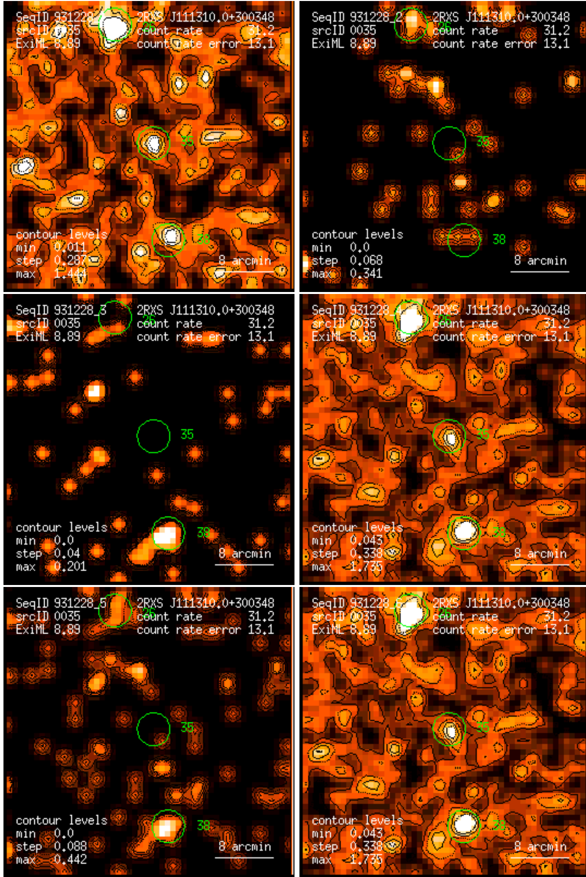
Figure 35: RASS 931228: detection 0035: band rate images, Gaussian filter: (1) PSPC channels 11 – 41, (2) 52 – 90, (3) 91 – 201, (4) 11 – 235, (5) 52 – 201, (6) 11 – 201. Broad band rates in counts/ks. Band rate contour levels in counts/ks/arcmin 2 .
