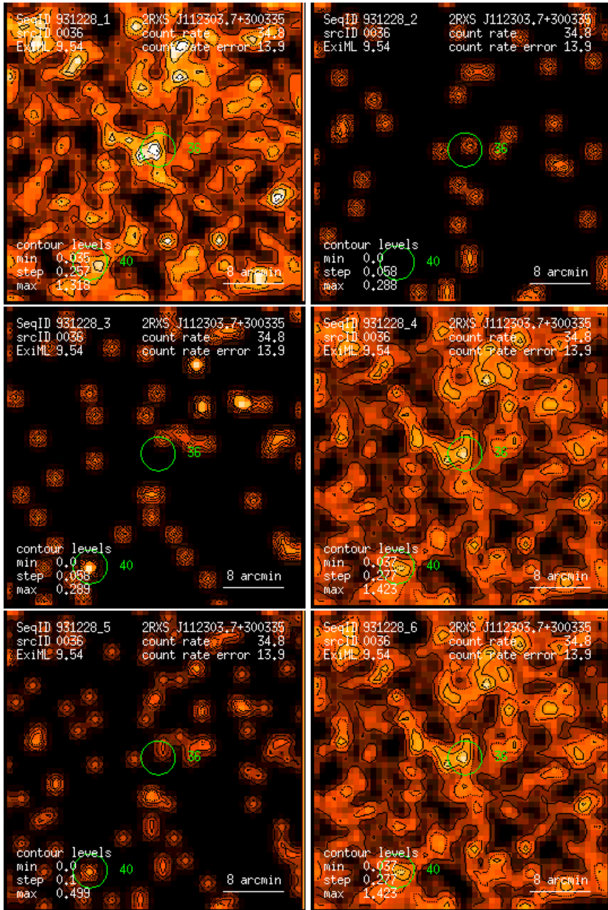
Figure 36: RASS 931228: detection 0036: band rate images, Gaussian filter: (1) PSPC channels 11 – 41, (2) 52 – 90, (3) 91 – 201, (4) 11 – 235, (5) 52 – 201, (6) 11 – 201. Broad band rates in counts/ks. Band rate contour levels in counts/ks/arcmin 2 .
