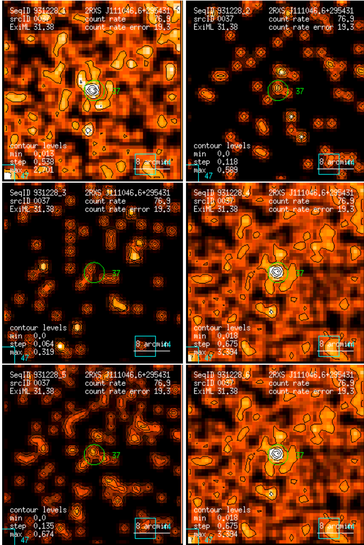
Figure 37: RASS 931228: detection 0037: band rate images, Gaussian filter: (1) PSPC channels 11 – 41, (2) 52 – 90, (3) 91 – 201, (4) 11 – 235, (5) 52 – 201, (6) 11 – 201. Broad band rates in counts/ks. Band rate contour levels in counts/ks/arcmin 2 .
