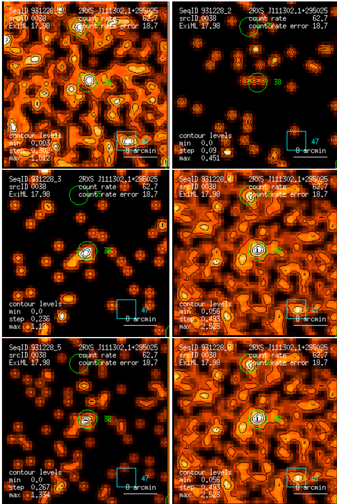
Figure 38: RASS 931228: detection 0038: band rate images, Gaussian filter: (1) PSPC channels 11 – 41, (2) 52 – 90, (3) 91 – 201, (4) 11 – 235, (5) 52 – 201, (6) 11 – 201. Broad band rates in counts/ks. Band rate contour levels in counts/ks/arcmin 2 .
