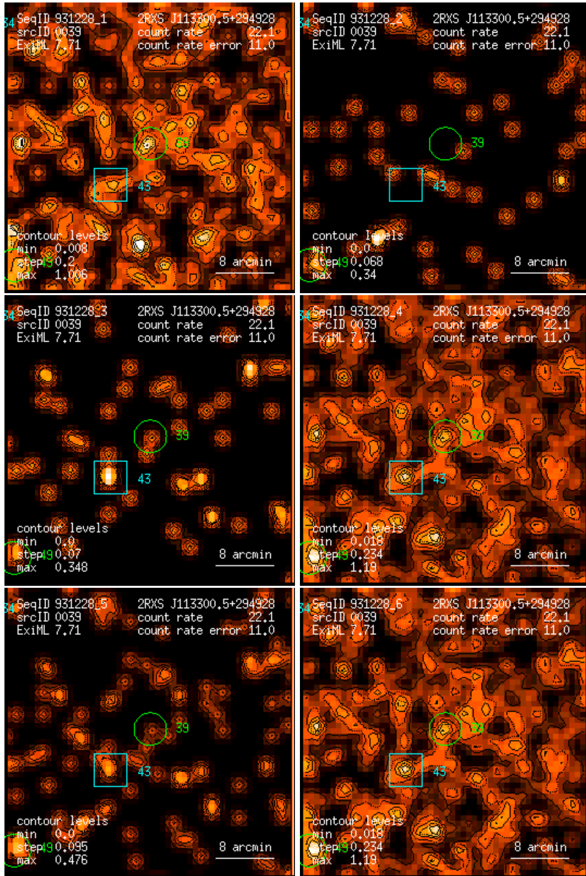
Figure 39: RASS 931228: detection 0039: band rate images, Gaussian filter: (1) PSPC channels 11 – 41, (2) 52 – 90, (3) 91 – 201, (4) 11 – 235, (5) 52 – 201, (6) 11 – 201. Broad band rates in counts/ks. Band rate contour levels in counts/ks/arcmin 2 .
