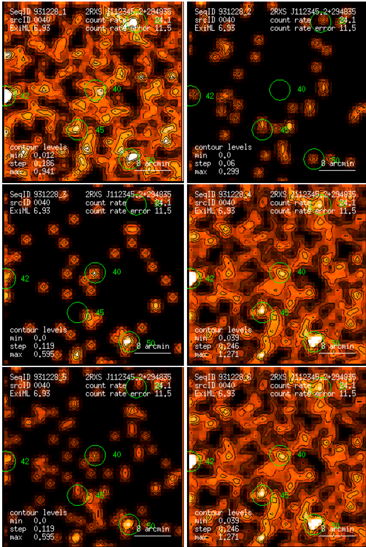
Figure 40: RASS 931228: detection 0040: band rate images, Gaussian filter: (1) PSPC channels 11 – 41, (2) 52 – 90, (3) 91 – 201, (4) 11 – 235, (5) 52 – 201, (6) 11 – 201. Broad band rates in counts/ks. Band rate contour levels in counts/ks/arcmin 2 .
