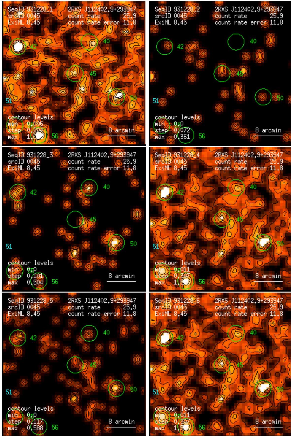
Figure 45: RASS 931228: detection 0045: band rate images, Gaussian filter: (1) PSPC channels 11 – 41, (2) 52 – 90, (3) 91 – 201, (4) 11 – 235, (5) 52 – 201, (6) 11 – 201. Broad band rates in counts/ks. Band rate contour levels in counts/ks/arcmin 2 .
