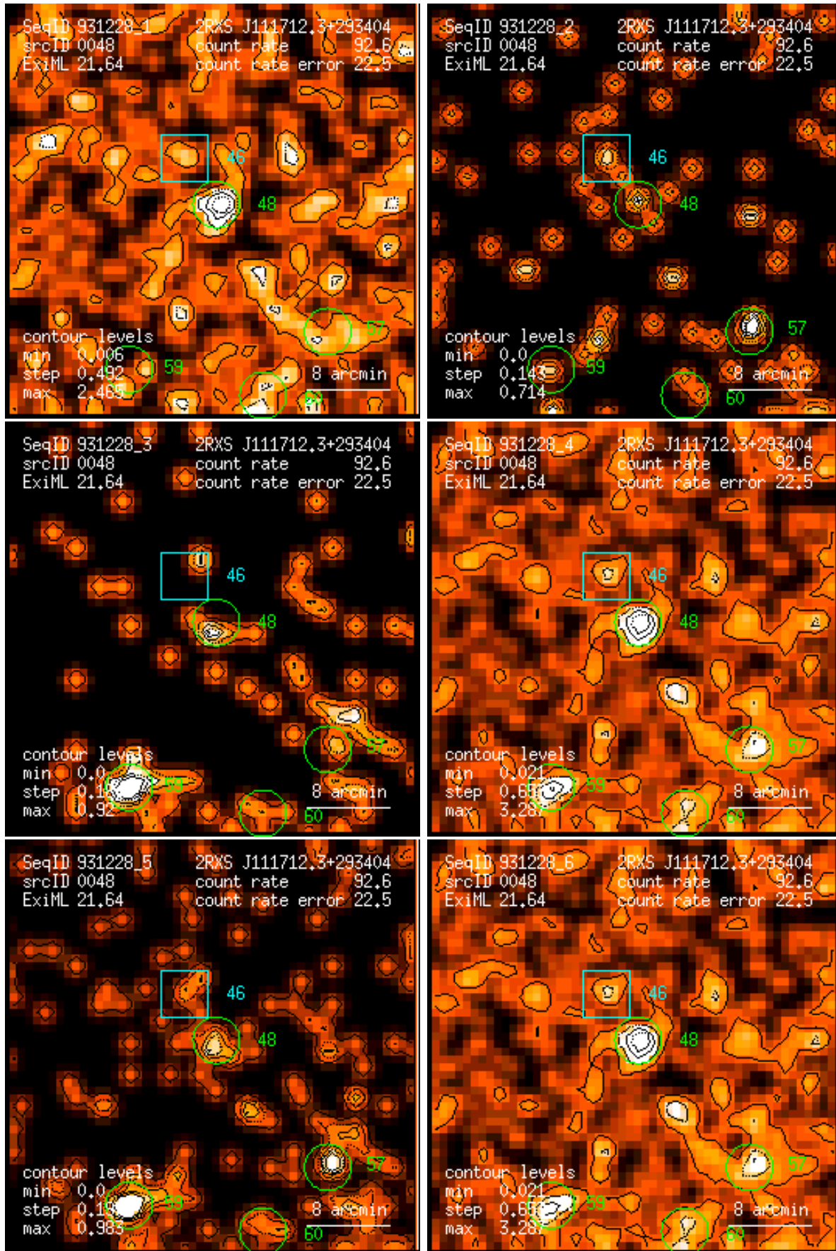
Figure 48: RASS 931228: detection 0048: band rate images, Gaussian filter: (1) PSPC channels 11 – 41, (2) 52 – 90, (3) 91 – 201, (4) 11 – 235, (5) 52 – 201, (6) 11 – 201. Broad band rates in counts/ks. Band rate contour levels in counts/ks/arcmin 2 .
