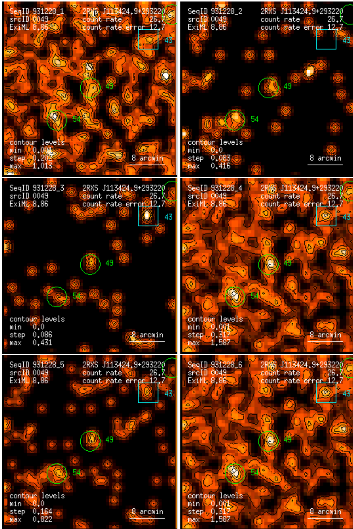
Figure 49: RASS 931228: detection 0049: band rate images, Gaussian filter: (1) PSPC channels 11 – 41, (2) 52 – 90, (3) 91 – 201, (4) 11 – 235, (5) 52 – 201, (6) 11 – 201. Broad band rates in counts/ks. Band rate contour levels in counts/ks/arcmin 2 .
