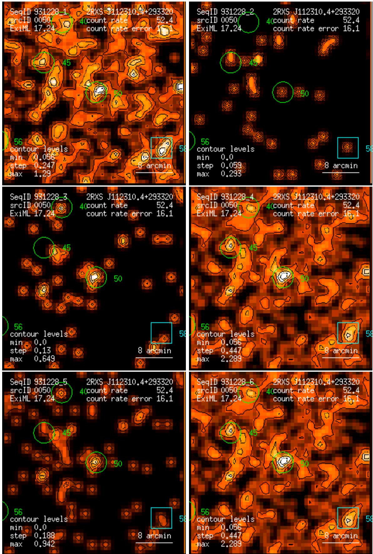
Figure 50: RASS 931228: detection 0050: band rate images, Gaussian filter: (1) PSPC channels 11 – 41, (2) 52 – 90, (3) 91 – 201, (4) 11 – 235, (5) 52 – 201, (6) 11 – 201. Broad band rates in counts/ks. Band rate contour levels in counts/ks/arcmin 2 .
