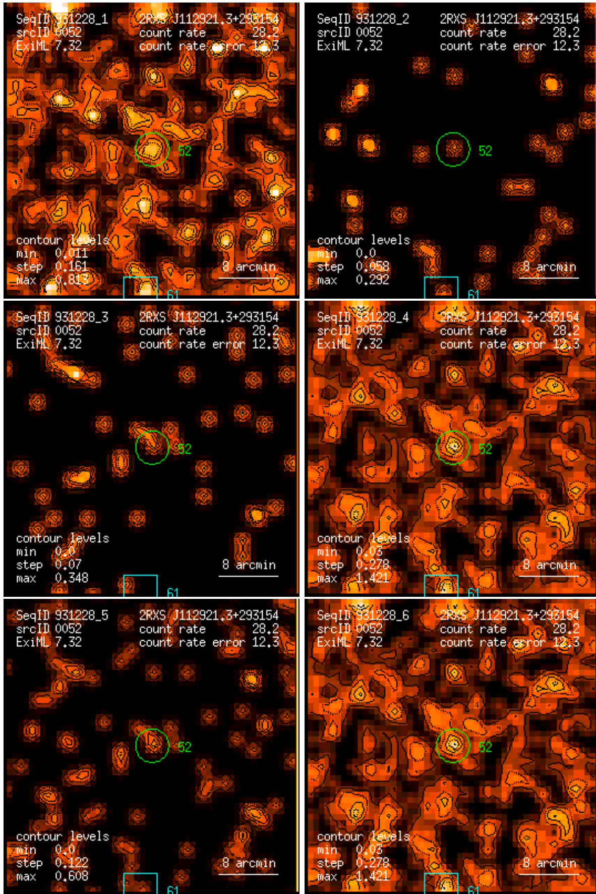
Figure 52: RASS 931228: detection 0052: band rate images, Gaussian filter: (1) PSPC channels 11 – 41, (2) 52 – 90, (3) 91 – 201, (4) 11 – 235, (5) 52 – 201, (6) 11 – 201. Broad band rates in counts/ks. Band rate contour levels in counts/ks/arcmin 2 .
