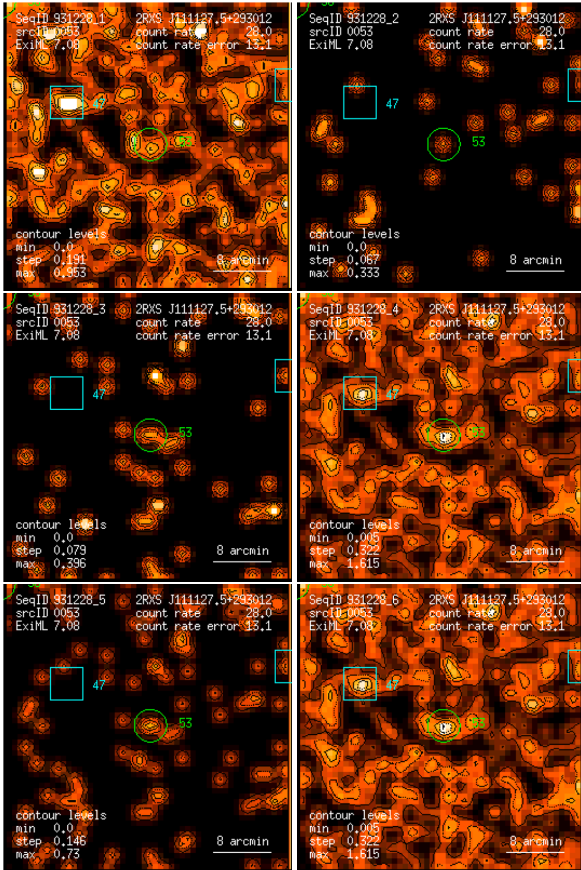
Figure 53: RASS 931228: detection 0053: band rate images, Gaussian filter: (1) PSPC channels 11 – 41, (2) 52 – 90, (3) 91 – 201, (4) 11 – 235, (5) 52 – 201, (6) 11 – 201. Broad band rates in counts/ks. Band rate contour levels in counts/ks/arcmin 2 .
