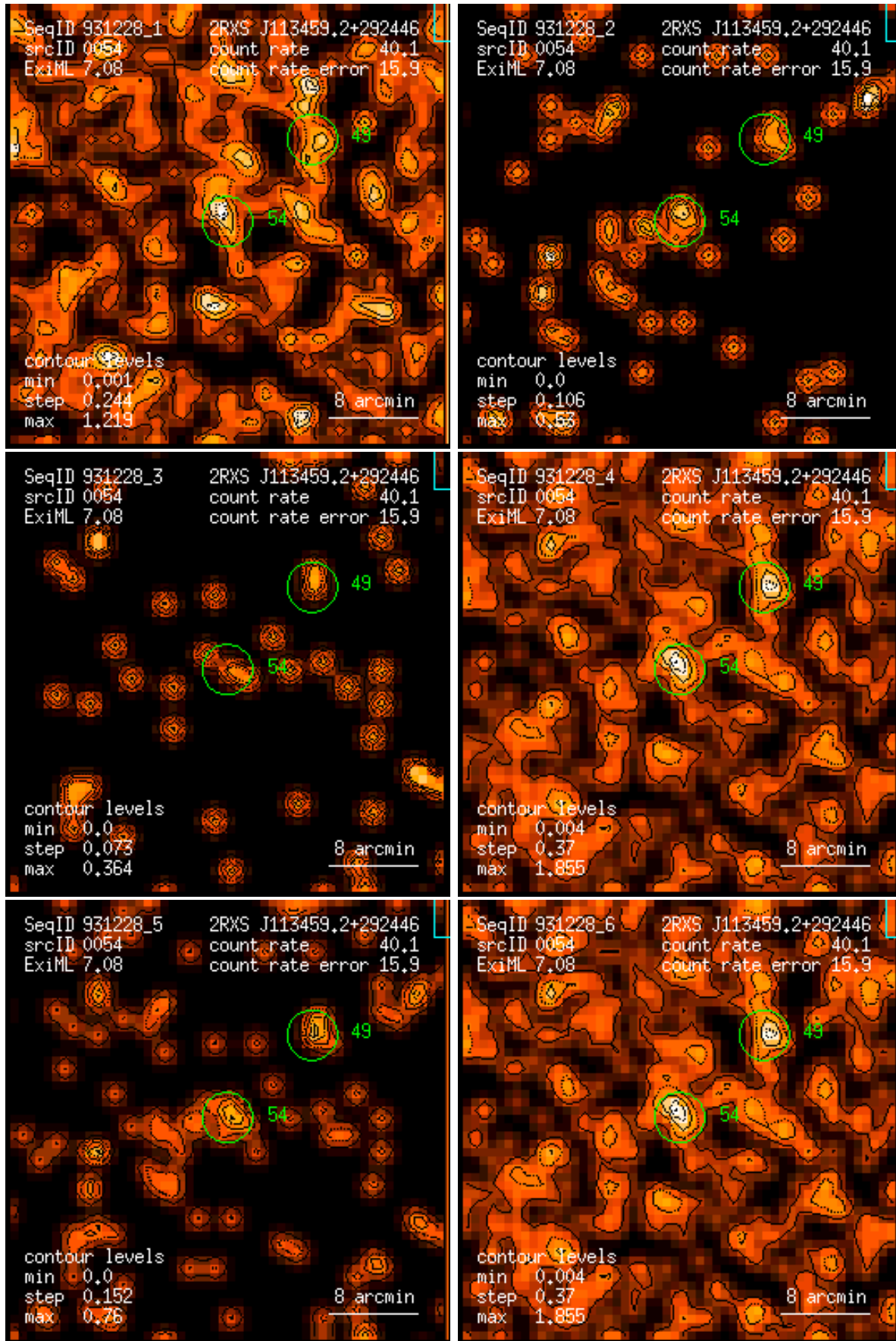
Figure 54: RASS 931228: detection 0054: band rate images, Gaussian filter: (1) PSPC channels 11 – 41, (2) 52 – 90, (3) 91 – 201, (4) 11 – 235, (5) 52 – 201, (6) 11 – 201. Broad band rates in counts/ks. Band rate contour levels in counts/ks/arcmin 2 .
