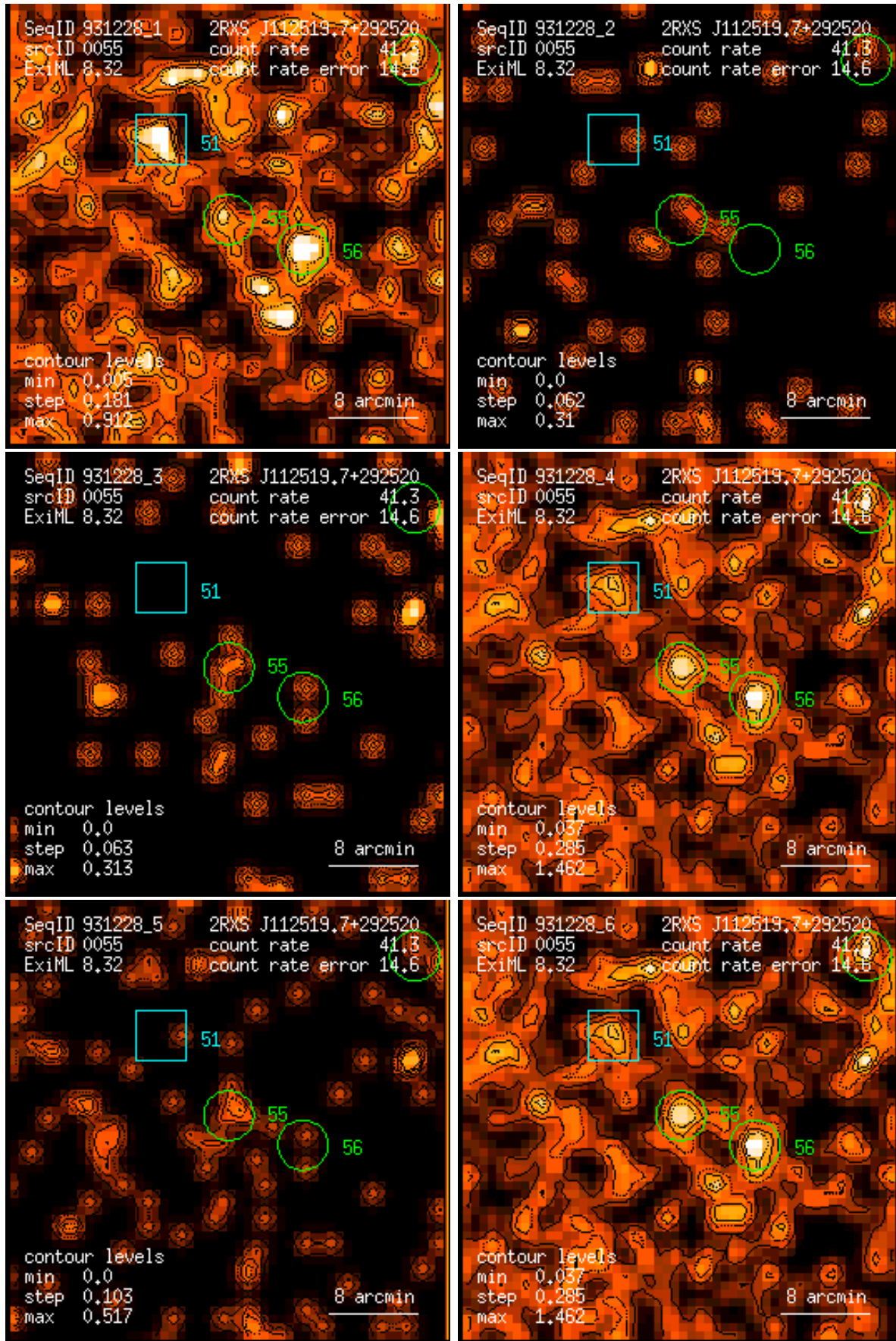
Figure 55: RASS 931228: detection 0055: band rate images, Gaussian filter: (1) PSPC channels 11 – 41, (2) 52 – 90, (3) 91 – 201, (4) 11 – 235, (5) 52 – 201, (6) 11 – 201. Broad band rates in counts/ks. Band rate contour levels in counts/ks/arcmin 2 .
