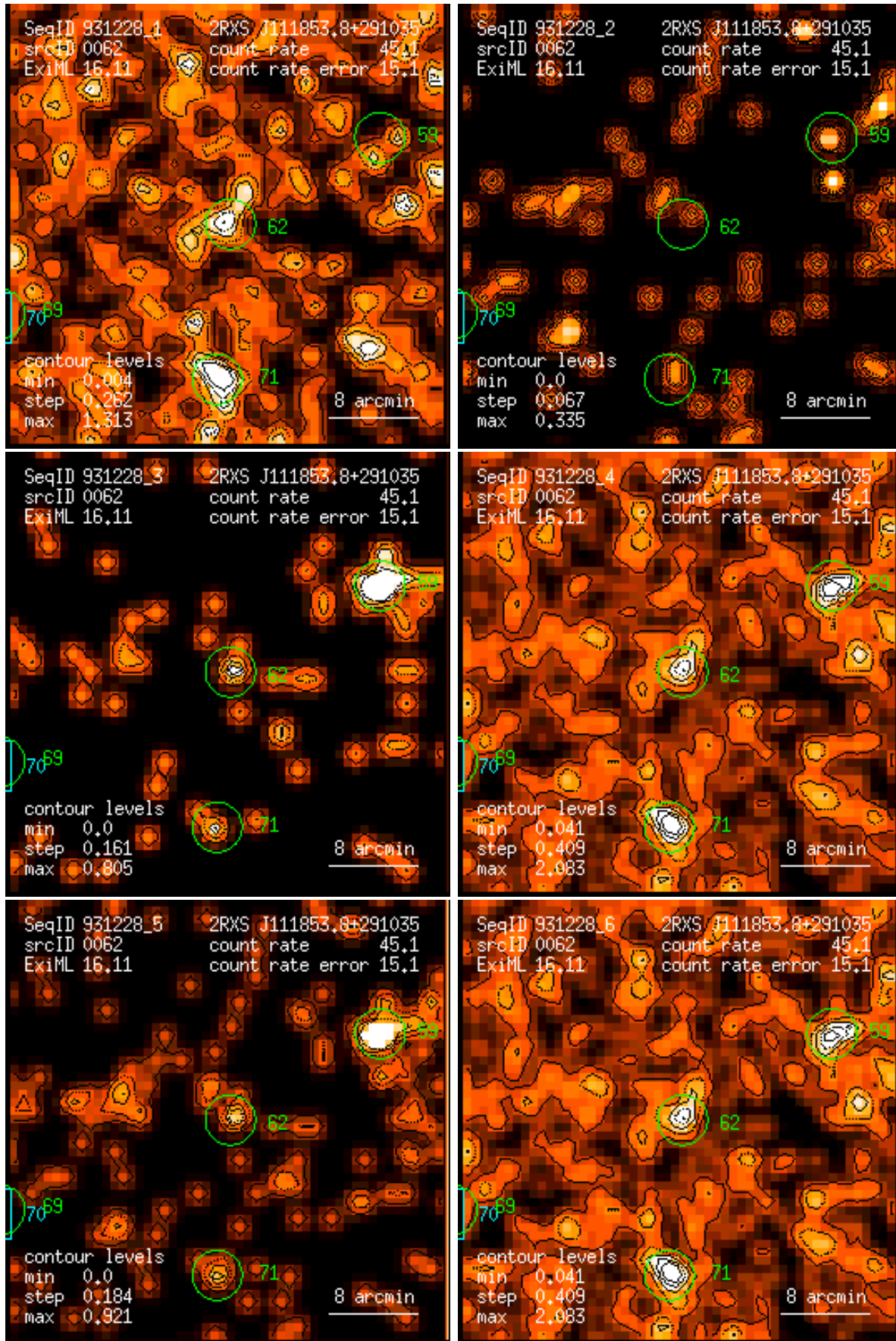
Figure 62: RASS 931228: detection 0062: band rate images, Gaussian filter: (1) PSPC channels 11 – 41, (2) 52 – 90, (3) 91 – 201, (4) 11 – 235, (5) 52 – 201, (6) 11 – 201. Broad band rates in counts/ks. Band rate contour levels in counts/ks/arcmin 2 .
