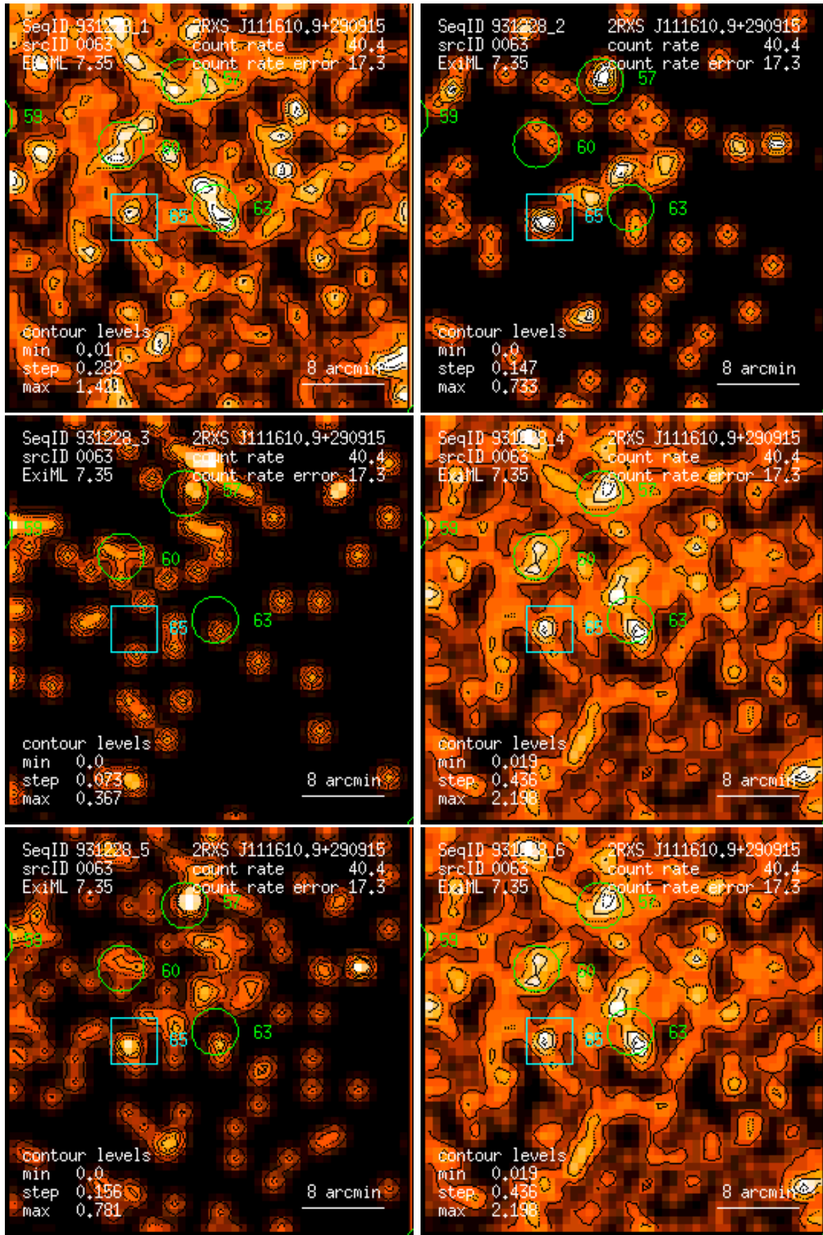
Figure 63: RASS 931228: detection 0063: band rate images, Gaussian filter: (1) PSPC channels 11 – 41, (2) 52 – 90, (3) 91 – 201, (4) 11 – 235, (5) 52 – 201, (6) 11 – 201. Broad band rates in counts/ks. Band rate contour levels in counts/ks/arcmin 2 .
