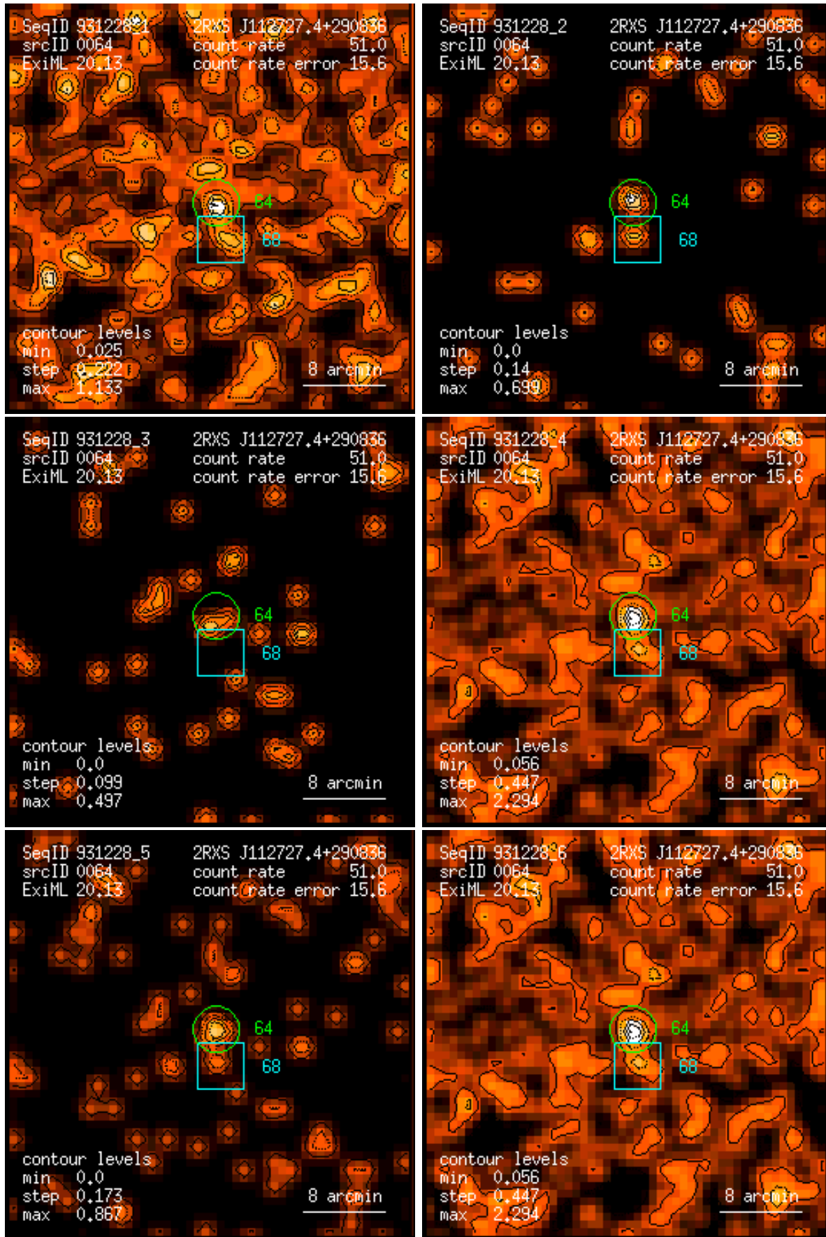
Figure 64: RASS 931228: detection 0064: band rate images, Gaussian filter: (1) PSPC channels 11 – 41, (2) 52 – 90, (3) 91 – 201, (4) 11 – 235, (5) 52 – 201, (6) 11 – 201. Broad band rates in counts/ks. Band rate contour levels in counts/ks/arcmin 2 .
